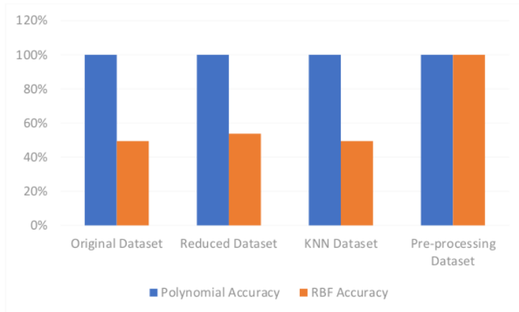
Fig 5. Dataset performance based on accuracy - percentage split
