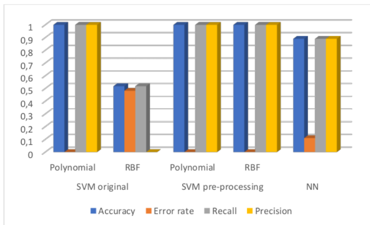
Fig. 6. Performance Polynomial and RBF kernel
