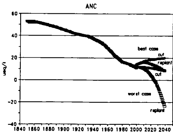
Figure 5.3b. Reconstructed historical streamwater alkalinity (meq/m 3 ) and predicted response under each scenario.
