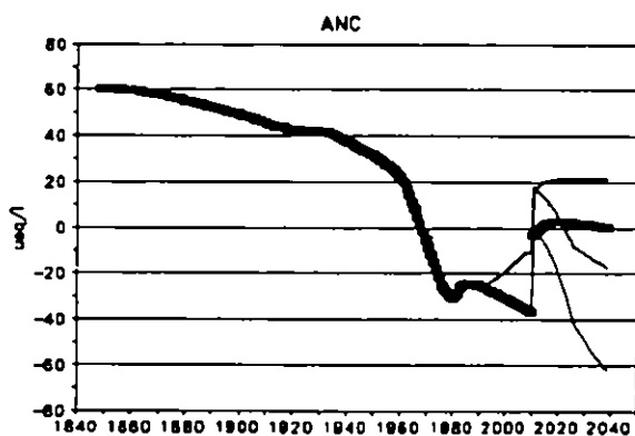
Figure 5.5b. Reconstructed historical streamwater alkalinity (meq/m 3 ) and predicted response under each scenario.
