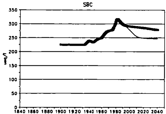
Figure 5.10c. Reconstructed historical streamwater sum of base cations (SBC meq/m 3 ) and predicted response under each scenario.
