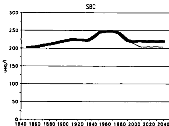
Figure 5.1c. Reconstructed historical streamwater sum of base cations (SBC meq/m 3 ) and predicted response under each scenario.
