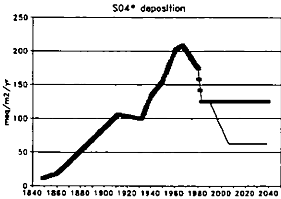
Figure 5.4a. Excess sulphate deposition (meq/m 2 /yr) used for best and worst case scenarios.
