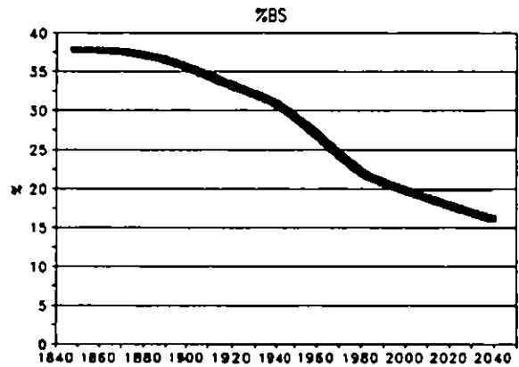
Figure 5.4d. Reconstructed historical soil base saturation (%) and predicted response under each scenario.
