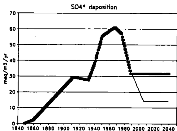
Figure 5.1a. Excess sulphate deposition (meq/m 2 /yr) used for best and worst case scenarios.
