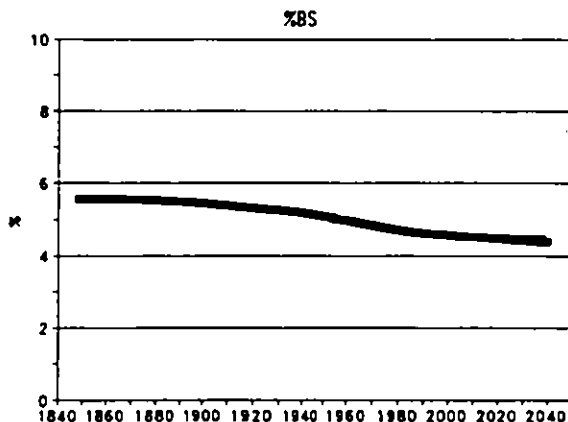
Figure 5.1d. Reconstructed historical soil base saturation (%) and predicted response under each scenario.
