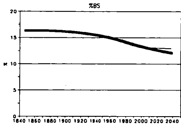
Figure 5.9d. Reconstructed historical soil base saturation (%) and predicted response under each scenario.
