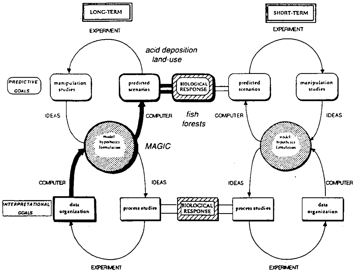
Figure 2. Diagrammatic sketch of the concept of ENCORE. Field measurements, process studies, model development and testing, manipulation experiments, and biological response are linked at the short and long term in small catchments (from Hornung et al. 1990). The highlights denote the links addressed here — data from catchments are used to calibrate the MAGIC model, which in turn generates predicted biological response to given scenarios.
