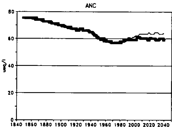
Figure 5.1b. Reconstructed historical streamwater alkalinity (meq/m 3 ) and predicted response under each scenario.
