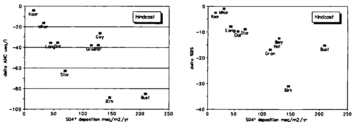
Figure 6.1. Change in streamwater ANC (left panel) and soil % base saturation (right panel) from pre-acidification (about 1840) to the present as reconstructed by MAGIC, and present-day excess-sulphate deposition at 10 ENCORE catchments.
