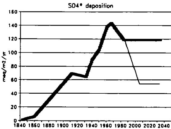
Figure 5.2a. Excess sulphate deposition (meq/m 2 /yr) used for best and worst case scenarios.
