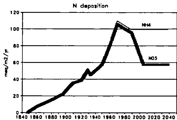
Figure 5.6e. Nitrogen deposition (meq/m 2 /yr) used for all scenarios.
