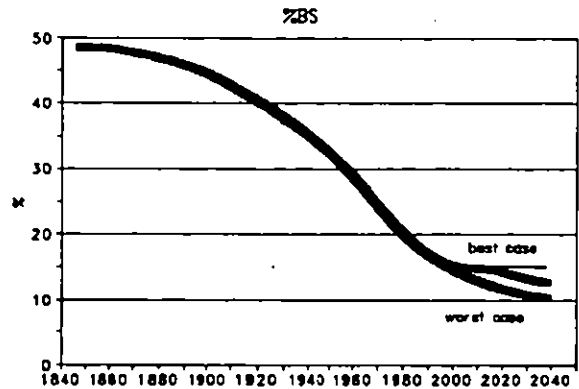
Figure 5.6d. Reconstructed historical soil base saturation (%) and predicted response under each scenario.
