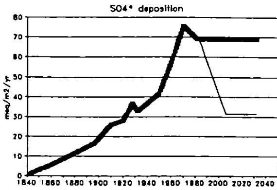
Figure 5.7a. Excess sulphate deposition (meq/m 2 /yr) used for best and worst case scenarios.
