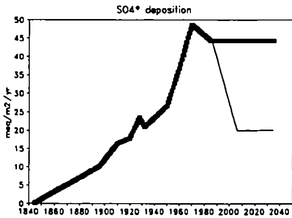
Figure 5.8a. Excess sulphate deposition (meq/m 2 /yr) used for best and worst case scenarios.
