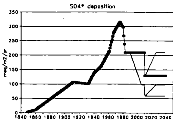
Figure 5.5a. Excess sulphate deposition (meq/m 2 /yr) used for best and worst case scenarios.
