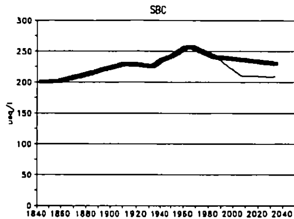
Figure 5.2c. Reconstructed historical streamwater sum of base cations (SBC meq/m 3 ) and predicted response under each scenario.
