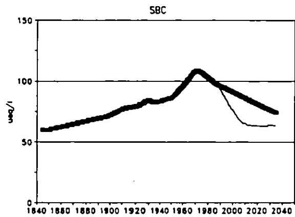
Figure 5.8c. Reconstructed historical streamwater sum of base cations (SBC meq/m 3 ) and predicted response under each scenario.
