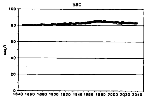
Figure 5.9c. Reconstructed historical streamwater sum of base cations (SBC meq/m 3 ) and predicted response under each scenario.
