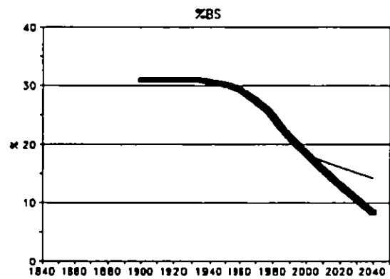
Figure 5.10d. Reconstructed historical soil base saturation (%) and predicted response under each scenario.
