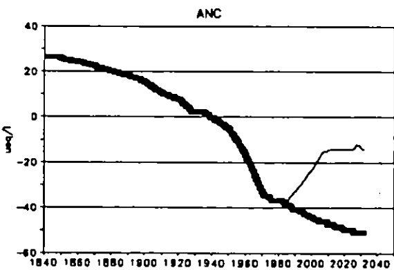
Figure 5.7b. Reconstructed historical streamwater alkalinity (meq/m 3 ) and predicted response under each scenario.
