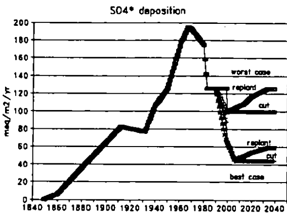
Figure 5.3a. Excess sulphate deposition (meq/m 2 /yr) used for best and worst case scenarios.
