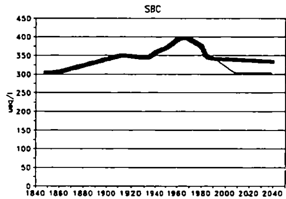
Figure 5.4c. Reconstructed historical streamwater sum of base cations (SBC meq/m 3 ) and predicted response under each scenario.
