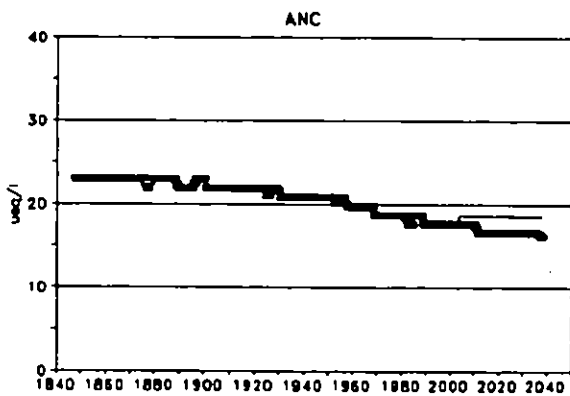
Figure 5.9b. Reconstructed historical streamwater alkalinity (meq/m 3 ) and predicted response under each scenario.
