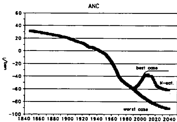
Figure 5.6b. Reconstructed historical streamwater alkalinity (meq/m 3 ) and predicted response under each scenario.
