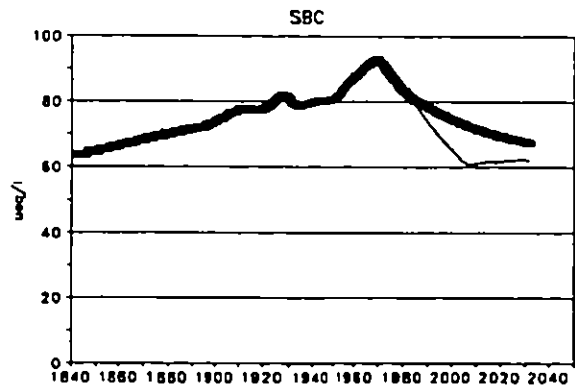
Figure 5.7c. Reconstructed historical streamwater sum of base cations (SBC meq/m 3 ) and predicted response under each scenario.
