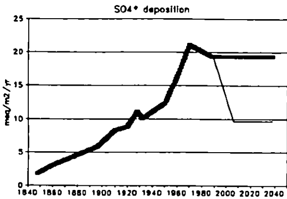
Figure 5.9a. Excess sulphate deposition (meq/m 2 /yr) used for best and worst case scenarios.
