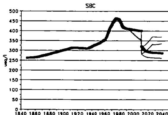
Figure 5.5c. Reconstructed historical streamwater sum of base cations (SBC meq/m 3 ) and predicted response under each scenario.
