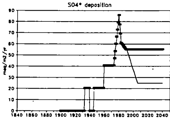
Figure 5.10a. Excess sulphate deposition (meq/m 2 /yr) used for best and worst case scenarios.
