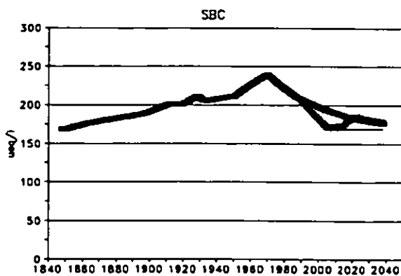
Figure 5.6c. Reconstructed historical streamwater sum of base cations (SBC meq/m 3 ) and predicted response under each scenario.
