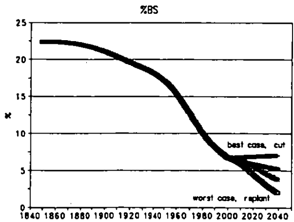
Figure 5.3d. Reconstructed historical soil base saturation (%) and predicted response under each scenario.
