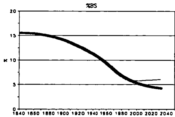
Figure 5.7d. Reconstructed historical soil base saturation (%) and predicted response under each scenario.
