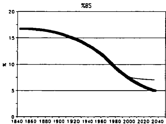
Figure 5.8d. Reconstructed historical soil base saturation (%) and predicted response under each scenario.
