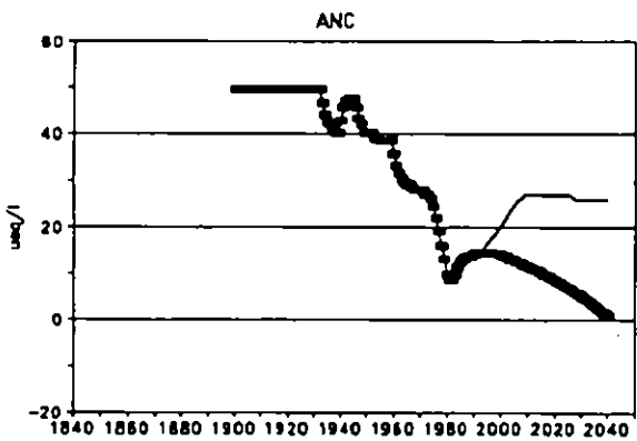
Figure 5.10b. Reconstructed historical streamwater alkalinity (meq/m 3 ) and predicted response under each scenario.
