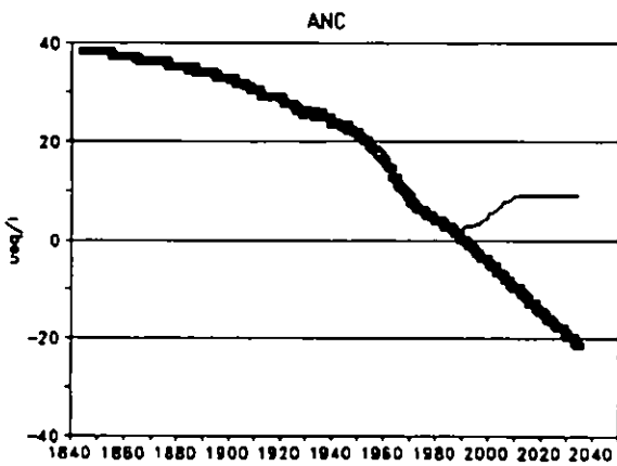
Figure 5.8b. Reconstructed historical streamwater alkalinity (meq/m 3 ) and predicted response under each scenario.
