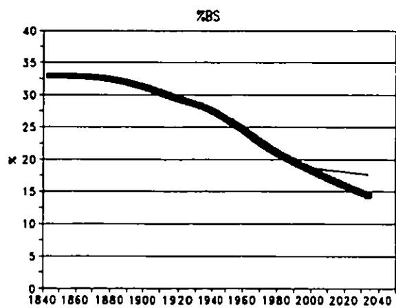
Figure 5.2d. Reconstructed historical soil base saturation (%) and predicted response under each scenario.
