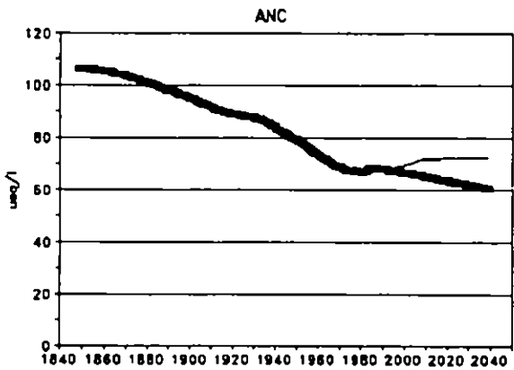
Figure 5.4b. Reconstructed historical streamwater alkalinity (meq/m 3 ) and predicted response under each scenario.
