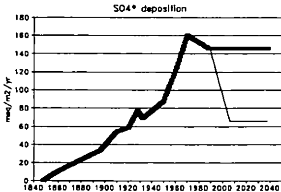
Figure 5.6a. Excess sulphate deposition (meq/m 2 /yr) used for best and worst case scenarios.
