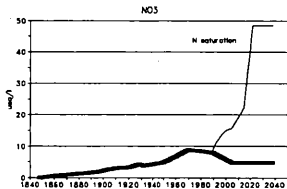
Figure 5.6f. Reconstructed historical streamwater nitrate (meq/m 2 ) and predicted response under constant nitrogen uptake and nitrogen saturation.
