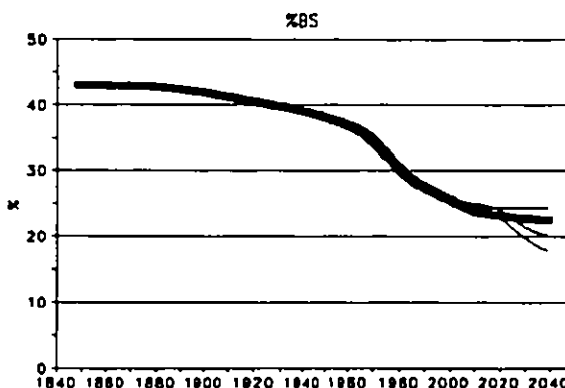
Figure 5.5d. Reconstructed historical soil base saturation (%) and predicted response under each scenario.
