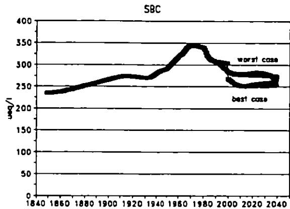
Figure 5.3c. Reconstructed historical streamwater sum of base cations (SBC meq/m 3 ) and predicted response under each scenario.
