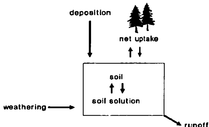
Figure 3. Schematic diagram of MAGIC. The pools of major chemical species in the catchment soil are central in MAGIC. Fluxes into and out of the catchment govern pool sizes; chemical equilibria between soil and soil solution determine the chemical composition of runoff. Terrestrial and aquatic biological response are related to soil and runoff chemistry, respectively.
