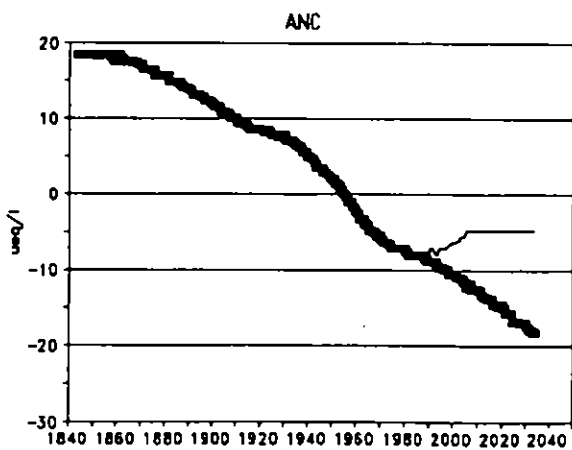
Figure 5.2b. Reconstructed historical streamwater alkalinity (meq/m 3 ) and predicted response under each scenario.
