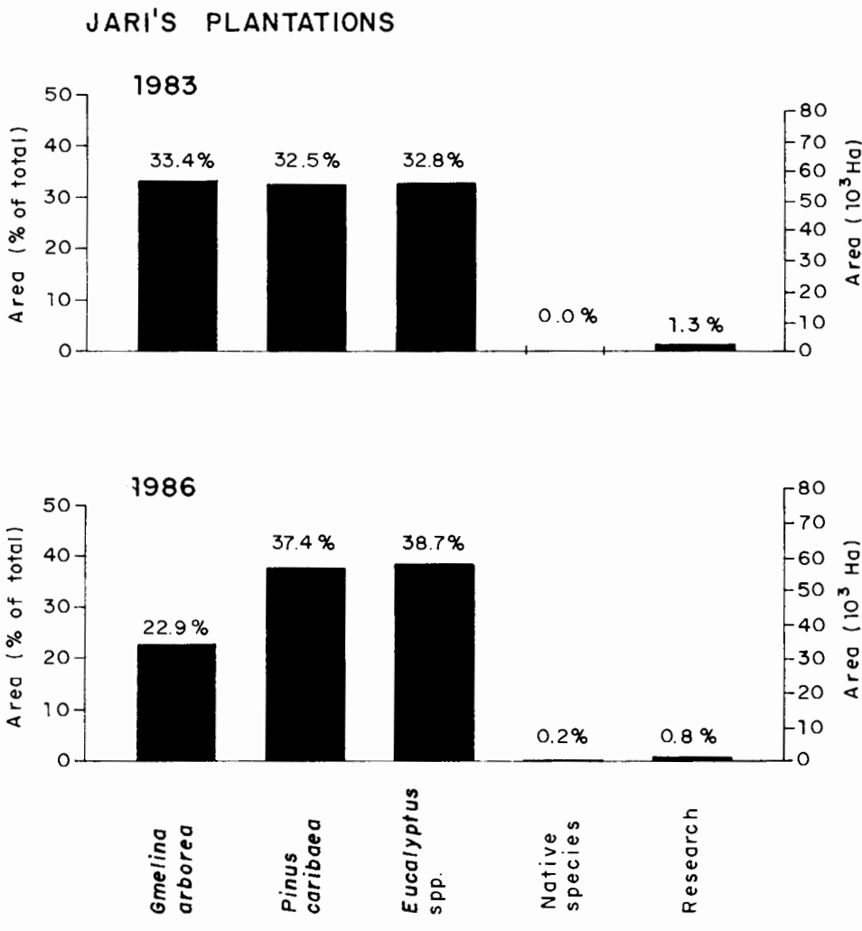
Fig. 2. Shift in silvicultural species at Jari.
