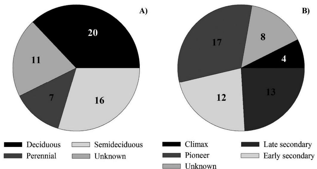
Figure 4. Classification according to deciduousness (A) and ecological groups (B) of the native tree species in the understory of Corymbia citriodora stand.
