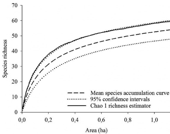
Figure 2. Mean species accumulation curve with respective confidence intervals and Chao 1 richness estimator for the native tree community in the Corymbia citriodora stand understory.
