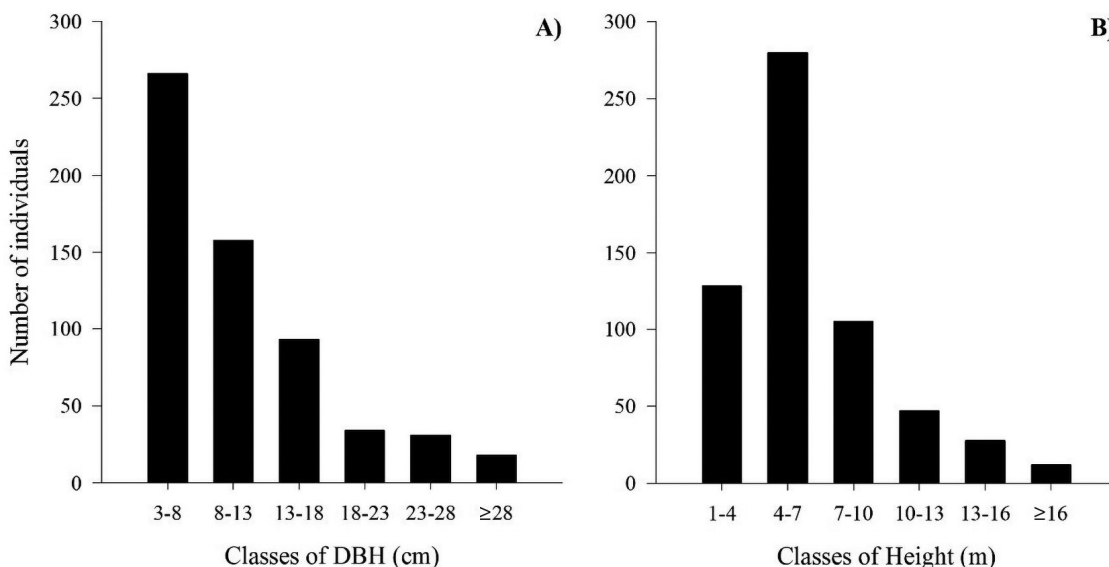
Figure 3. Diameter (A) and height (B) distributions of the native tree species in the understory of Corymbia citriodora stand. DBH: diameter at breast height.
