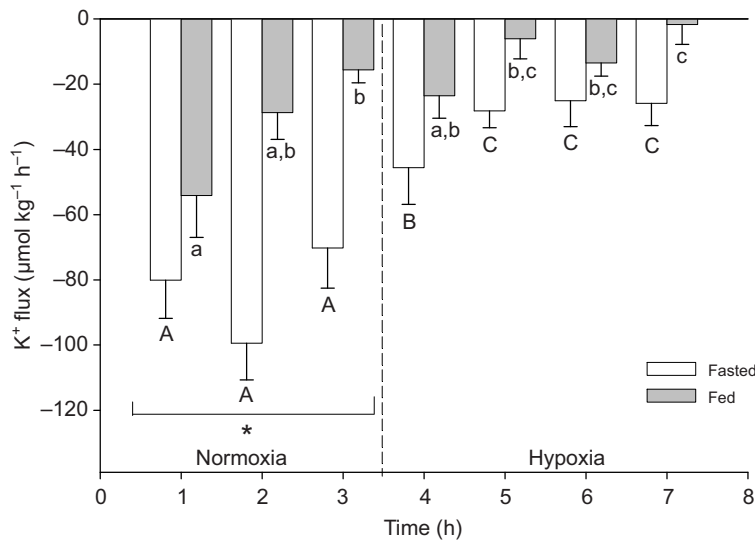
Fig. 3. Changes in net flux rates of K + in oscar fish that were either fasted for 10–14 days (white bars) or fed up to 24 h before the start of the experiment (grey bars). The fish were exposed to normoxia (P O 2 =130–150 Torr) followed by acute hypoxia (P O 2 =10–20 Torr). Data are means ± 1 s.e.m. (N=9–12). Asterisk indicates a significant difference (*P≤0.05) between normoxic fed and fasted fish at the same time period, and different letters indicate a significant difference (P≤0.05) between normoxic and hypoxic flux rates (uppercase for fasted fish, lowercase for fed fish).
