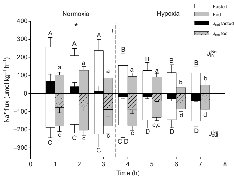
Fig. 2. Changes in unidirectional ( J_{\text{out}}^{\text{Na}} , J_{\text{in}}^{\text{Na}} ) and net flux rates ( J_{\text{net}}^{\text{Na}} ) of \text{Na}^+ in oscars that were either fasted for 10–14 days or fed up to 24 h before the start of the experiment. J_{\text{out}}^{\text{Na}} values are downward bars (white for fasted and grey for fed fish), J_{\text{in}}^{\text{Na}} values are upward bars (white for fasted and grey for fed fish) and J_{\text{net}}^{\text{Na}} values are black (fasted fish) or grey hatched bars (fed fish). The fish were exposed to normoxia ( P_{\text{O}_2}=130\text{--}150 Torr) followed by acute hypoxia ( P_{\text{O}_2}=10\text{--}20 Torr). Data are means \pm 1 s.e.m. ( N=9\text{--}12 ). Asterisk indicates a significant difference ( *P\leq 0.05 ) between normoxic fed and fasted fish at the same time period, and letters indicate a significant difference ( P\leq 0.05 ) between normoxic and hypoxic flux rates (uppercase for fasted fish, lowercase for fed fish).
