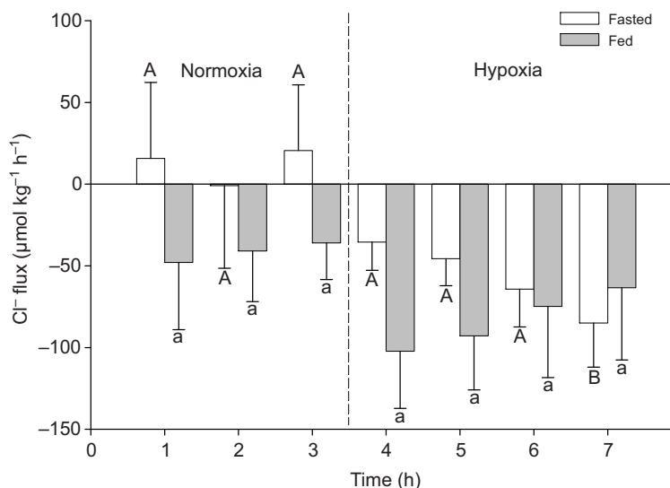
Fig. 4. Changes in net flux rates of Cl - in oscar fish that were either fasted for 10–14 days (white bars) or fed up to 24 h before the start of the experiment (grey bars). The fish were exposed to normoxia (P O 2 =130–150 Torr) followed by acute hypoxia (P O 2 =10–20 Torr). Data are means ± 1 s.e.m. (N=9–12). Different letters indicate a significant difference (P≤0.05) between normoxic and hypoxic flux rates (uppercase for fasted fish, lowercase for fed fish).
