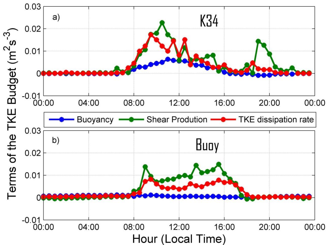
Figure 5. Diurnal cycle of the terms of the TKE budget for K34 (a) and CU (b) sites.
