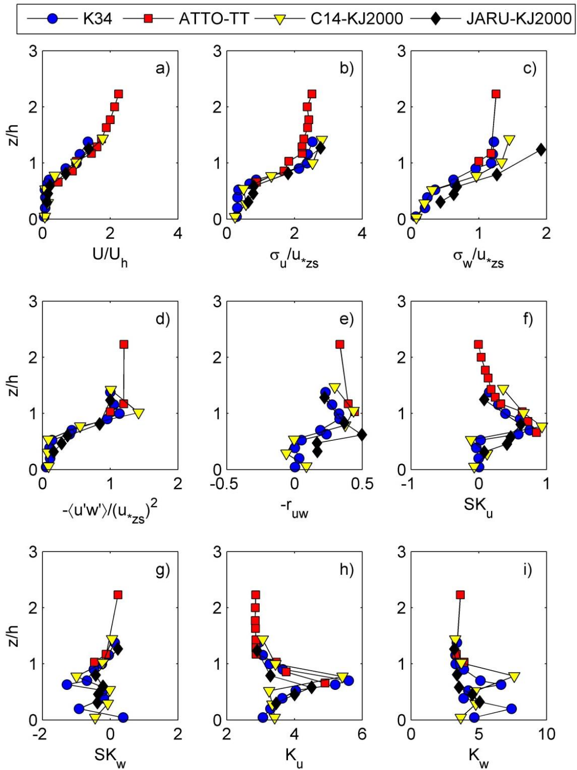
Figure 2. Vertical profiles in (a) U/U_h ; (b) \sigma_u/u_{*zs} ; (c) \sigma_w/u_{*zs} ; (d) -\langle u'w' \rangle / (u_{*zs})^2 ; (e) -r = -\overline{u'w'}/(\sigma_u\sigma_w) ; (f) Sk_u = \overline{(u')^3}/\sigma_u^3 , (g) Sk_w = \overline{(w')^3}/\sigma_w^3 ; (h) k_u = \overline{(u')^4}/\sigma_u^4 ; e (i) k_w = \overline{(w')^4}/\sigma_w^4 , for K34, ATTO, C14 and Jaru sites. Table 3 provides a summary of the heights at which the u_{*zs} measurements were performed.
