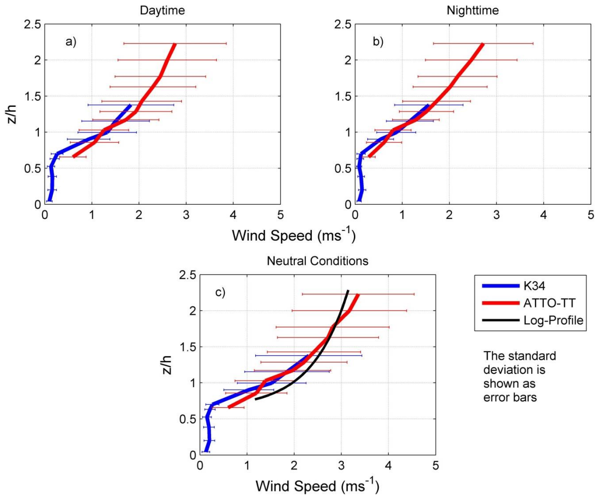
Figure 3. Vertical wind profile for K34 (blue line) and ATTO triangular tower (red line). The horizontal lines represent the standard deviation for each measurement point. The logarithmic profile was obtained through the equation \bar{u} = \frac{u_*}{k} \ln\left(\frac{z-d}{z_0}\right) , where k is von Karman's constant, z_0 = \frac{1}{30}h is roughness length and d = 0.75h is displacement height [17].
