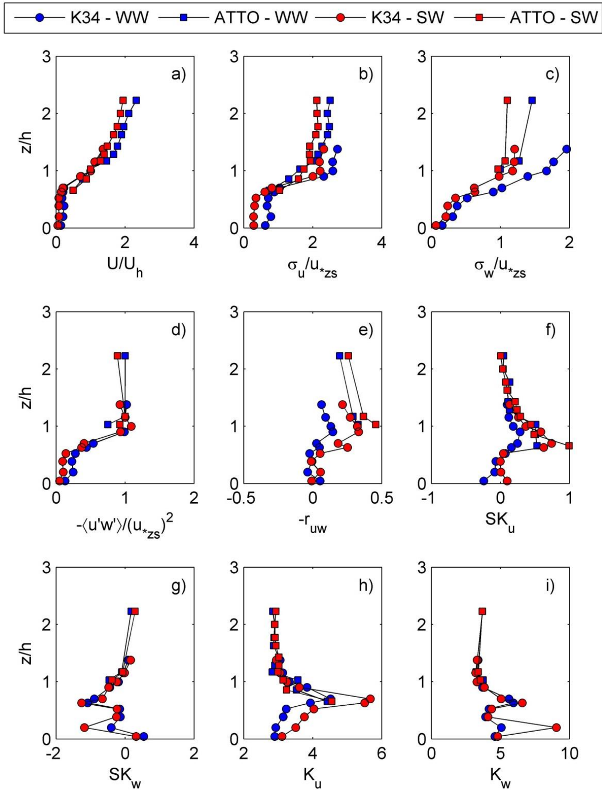
Figure 4. Vertical profiles in (a) U/U_h ; (b) \sigma_u/u_{*zs} ; (c) \sigma_w/u_{*zs} ; (d) -\langle u'w' \rangle / (u_{*zs})^2 ; (e) -r = -\overline{u'w'}/(\sigma_u\sigma_w) ; (f) Sk_u = \overline{(u')^3}/\sigma_u^3 , (g) Sk_w = \overline{(w')^3}/\sigma_w^3 ; (h) k_u = \overline{(u')^4}/\sigma_u^4 ; e (i) k_w = \overline{(w')^4}/\sigma_w^4 , for K34 and ATTO sites. The heights at which the u_{*zs} measures were performed are summarized in Table 3. Daytime period under weak wind (WW, blue color) and strong wind (SW, red color).
