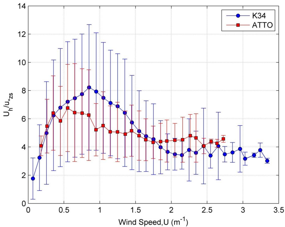
Figure 3. Relationship between wind speed at h height and U_h/u_{*zs} ratio for both K34 ATTO site. The standard deviation is shown as error bars.
