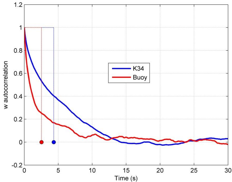
Figure 2. Correlogram of the vertical velocity. Each curve refers to 30 minutes data from both sites. The circles represent the \Lambda_w values for both CU (red) and K34 (blue) sites. Such values are numerically equal to the areas formed under the curves of each site.
