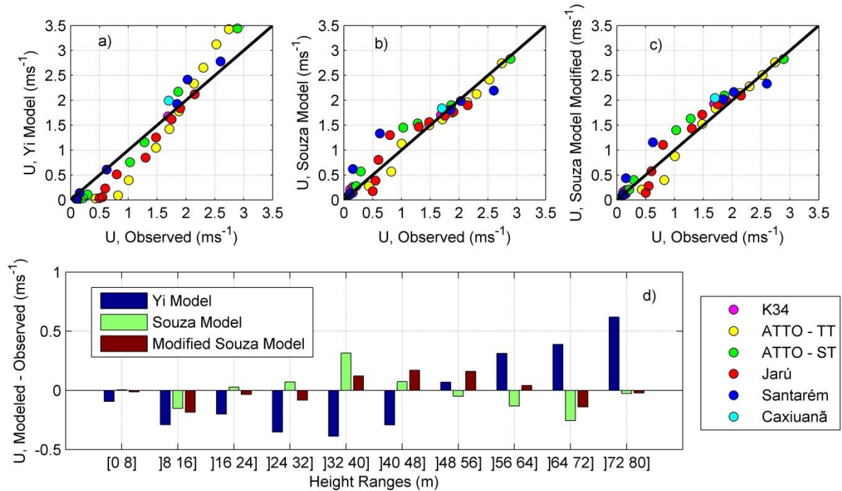
Figure 6. Wind speed (U) observed versus modeled for the three models used in this study (a, b and c). Part d shows the modeled minus observed wind speed for different intervals of heights, above and below the forest canopy.
