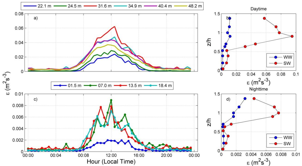
Figure 7. \epsilon diurnal cycle in a and c. Vertical \epsilon profile for weak and strong wind conditions during daytime (b) and nighttime (d) periods.
