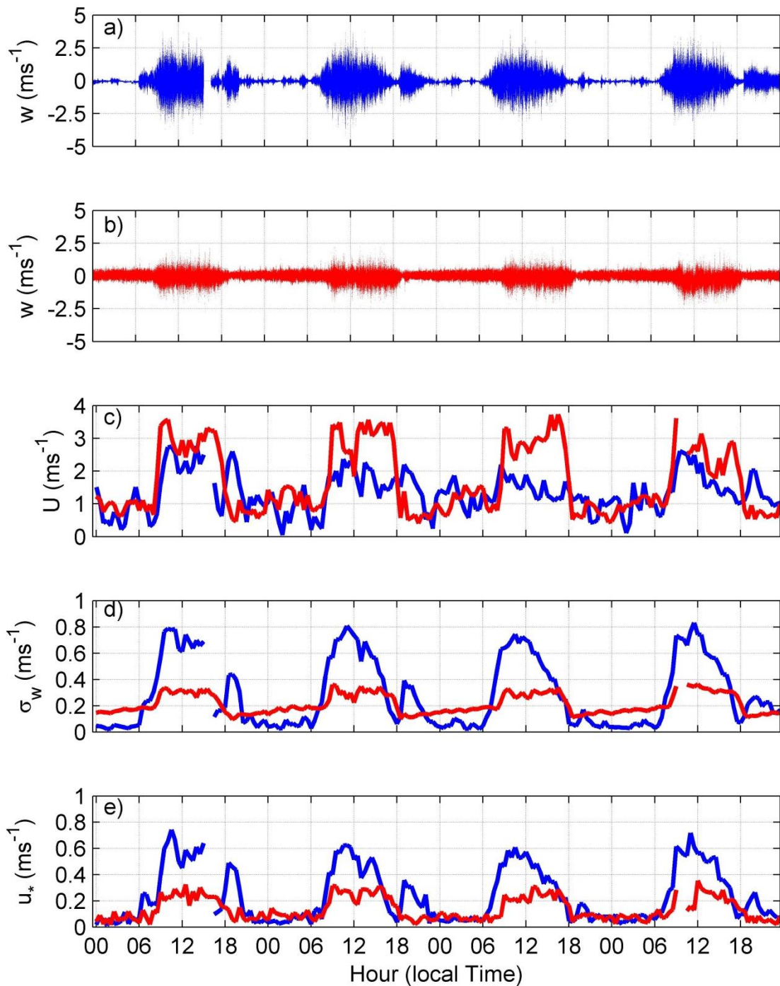
Figure 3. Time series of the w wind component (a and b), mean wind (c), w standard deviation (d) and friction velocity (e) for K34 (blue) and CU (red) sites.
