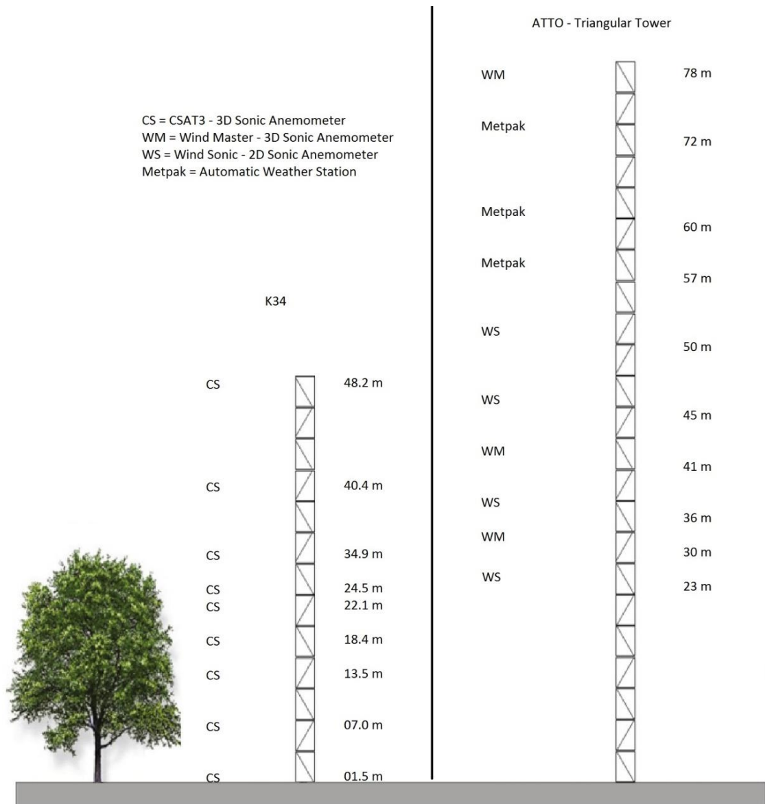
Figure 1. Illustrative figure representing the measurement instruments installed in the K34 and ATTO experimental sites.
