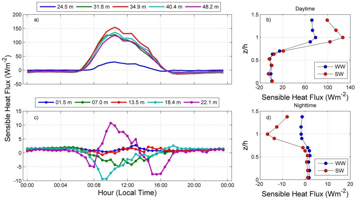
Figure 6. Diurnal cycle of the sensible heat flux for different heights for both inside and above the canopy forest for the K34 site in a and c. Sensible heat flux profile for weak (WW) and strong (SW) wind conditions for daytime (b) and nighttime (d) periods.
