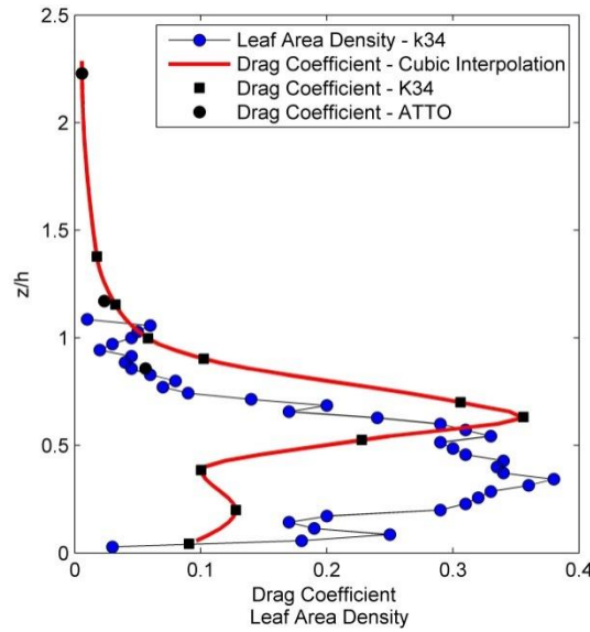
Figure 2. Leaf area density vertical profile (source: Tóta et al. [34]) and drag coefficient profile.
