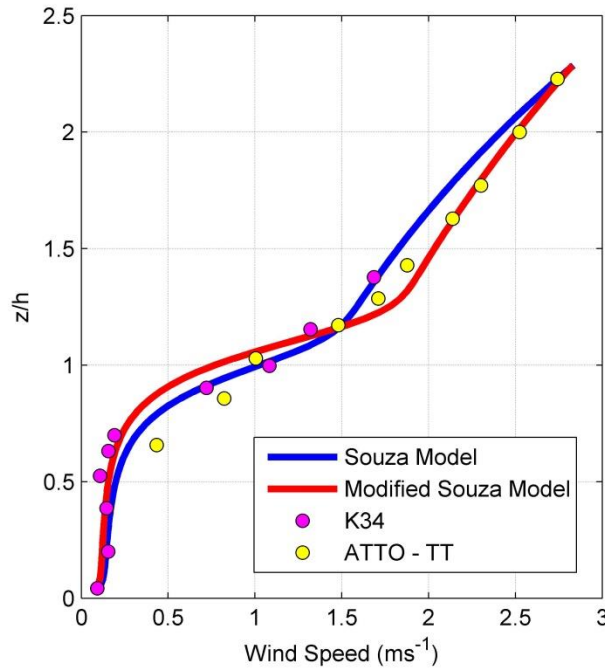
Figure 4. Observed and modeled vertical wind profiles.
