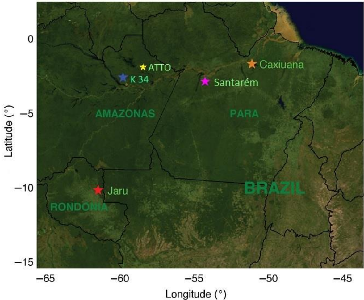
Figure 1. Experimental sites located in the Amazon (Source: Adapted from Zeri et al. [31])
