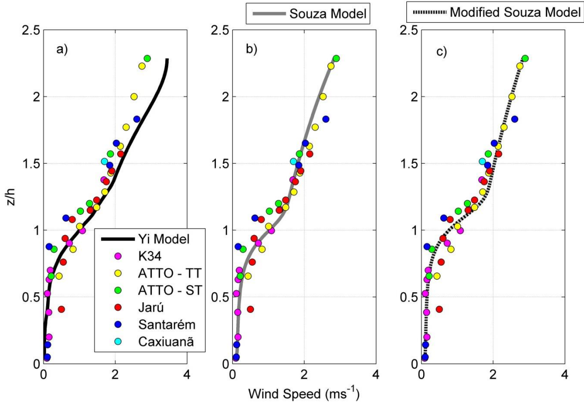
Figure 5. Vertical wind profile observed and modeled in different experimental sites in the Amazon.
