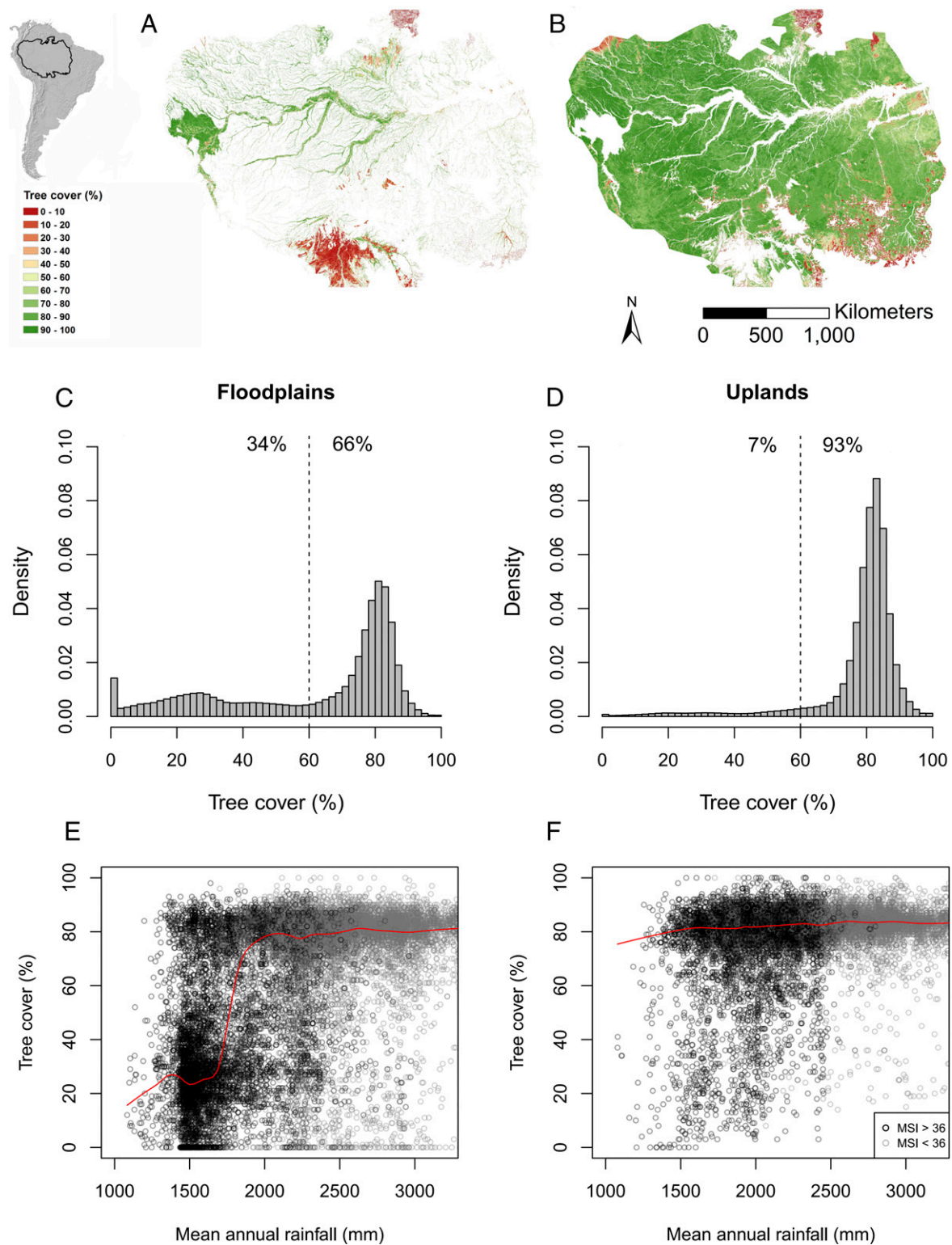
Fig. 1. Distribution of tree cover across the Amazon basin. (A) Floodplains and (B) uplands separated by the wetlands' mask (15). Deforested areas were excluded ( SI Methods ). Density distributions of tree cover for (C) floodplains and (D) uplands. A cutoff at 60% tree cover (dashed lines) separates forest from savanna (3), and percentage values are the proportion in each state. Relation between mean annual rainfall and tree cover for (E) floodplains and (F) uplands. Markham seasonality index values >36 (black circles) and <36 (gray circles) are shown. Red lines are fitted locally weighted scatterplot smoothing (LOWESS). Circles are 15,000 data points randomly sampled for each case.
