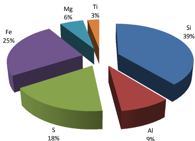
Figure 31. Average bulk elemental concentrations (in weight-percent) of \text{PM}_{2.5} aerosols collected at 80 m height between 7 March and 21 April 2012.
