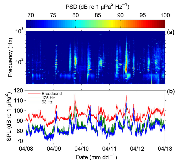
Fig. 4. Time-series analysis of ship passages recorded using an autonomous marine acoustic recording unit (MARU; developed by the Bioacoustics Research Program at Cornell University) in Stellwagen Bank National Marine Sanctuary, Massachusetts Bay, USA, in April 2010. Sampling rate: 2 kHz. (a) Spectrogram composed of PSDs with 1-s time segments; (b) 63- and 125-Hz 1/3-octave bands and broadband (0.2–1 kHz) SPL. Analysis parameters: 1-s time segments averaged to 60-s resolution via the Welch method.
