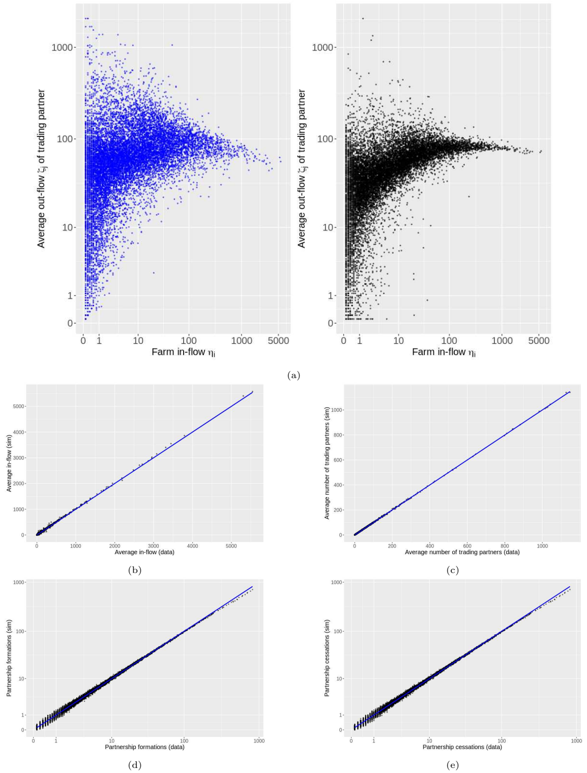
Figure 1: Model fit to data. For model with modifications to partnership formation and cessation rates. Panel (a) shows the average out-flow, \zeta_j , of farms' trading partners, where blue points are obtained from data, and points from stochastic simulation, where simulations are performed using Gillespie Stochastic Simulation Algorithm. Bottom four panels show comparisons of simulation output and data for four statistics: annual in-flow (b), annual number of concurrent trading partners (c), annual number of partnership formations (d), and annual number of partnership cessations (e).
