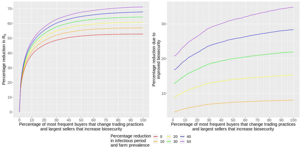
Figure 5: Comparing biosecurity with changes to trade patterns. Percentage reduction in R_0 (disease parameters \lambda = 0.25 and \gamma = 0.2 ) for targeted changes to both trading practices and improved biosecurity (left), and due solely to targeted improvements to biosecurity (right). In both cases, x -axes indicate what percentage of the most frequent buyers adopt trade changes and largest sellers improve biosecurity.
