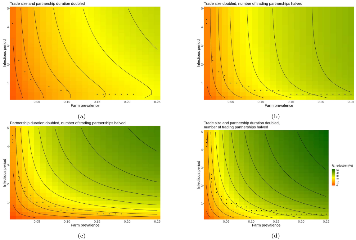
Figure 3: Reducing endemic disease burden. The percentage reduction in the system average R_0 for a range of disease parameterisations under specific trading and partnership dynamics changes, when compared with values of R_0 for current trading patterns in the Scottish trade system. Black points represent disease parameterisations in which R_0 > 1 before changes, and R_0 < 1 after changes are implemented.
