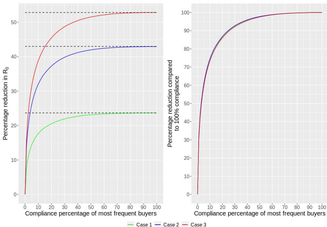
Figure 4: Targeting high risk farms. Percentage reduction in R_0 compared to: current trading patterns (left); and 100% adoption of new trading patterns (right). The new trading patterns are those shown in the bottom right panel of Figure 3d, which provides percentage reduction at 100% (dashed lines). In both panels the x -axis indicates what percentage of the most frequent buyers (those making the largest number of trades annually) are adopting these changes. Different disease parameterisations are shown with dashed lines representing values of R_0 for: Case 1) \lambda = 0.06 , \gamma = 1 ; Case 2) \lambda = 0.15 , \gamma = 0.4 ; and Case 3) \lambda = 0.25 , \gamma = 0.2 . Initial R_0 values for current trading patterns are: Case 1) R_0 = 1.19 , Case 2) R_0 = 4.92 , and Case 3) R_0 = 11.43 .
