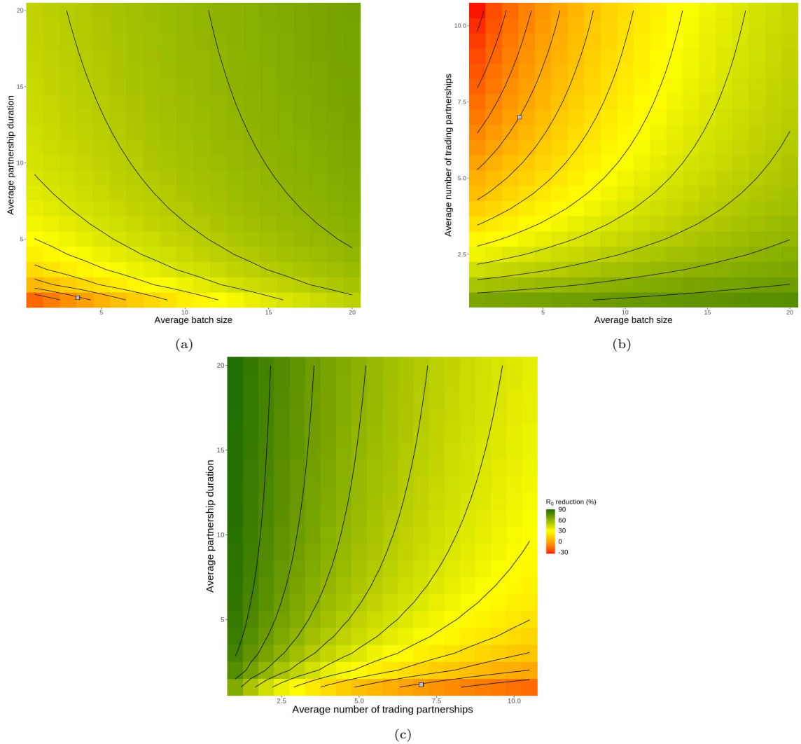
Figure 2: Impact of trade behaviour and partnership dynamics. Percentage change in R_0 for a persistent and high prevalence disease ( \lambda = \gamma = 0.2 ) due to changes in the dynamics of trade and trade partnerships compared with the current dynamics of the Scottish trade system (grey squares). We consider changes to batch size and partnership duration (a), batch size and number of concurrent trading partners (b), and number of concurrent trading partners and partnership duration (c).
