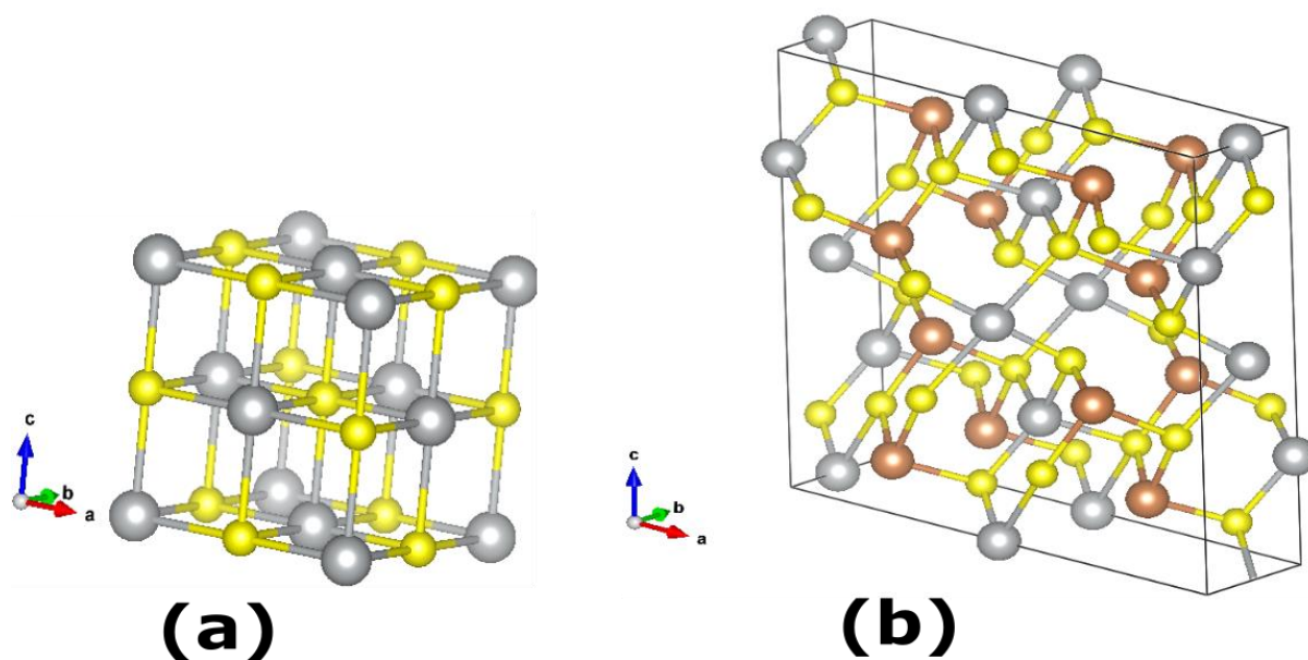
Fig. 1 (a) Cubic cuboargyrite \beta -AgSbS 2 reported by Geller and Wernick, with the silver and antimony indistinguishable 33 . (b) monoclinic \alpha -AgSbS 2 miargyrite was obtained by Smith 34 . In all cases silver atoms (Ag) are represented by silver spheres, Antimony (Sb) by brown spheres and S by yellow spheres.
