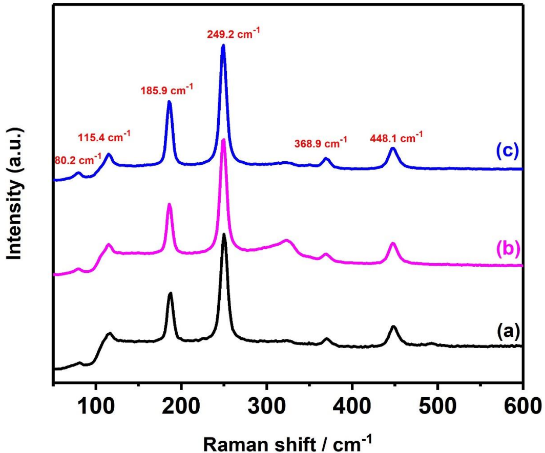
Fig. 5 Raman spectra of \text{AgSbS}_2 powders synthesised at different temperatures (a) 400\text{ }^\circ\text{C} , (b) 450\text{ }^\circ\text{C} and (c) 500\text{ }^\circ\text{C} for 1 h under nitrogen.
