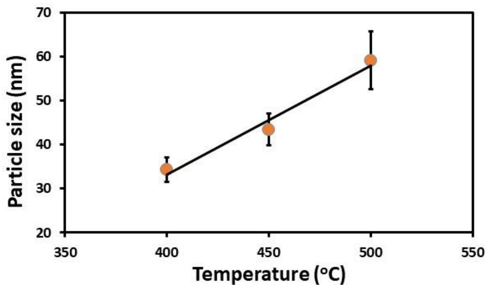
Fig. 4 Average crystallite domain size of \text{AgSbS}_2 powders calculated using Scherrer's equation as a function of synthesis temperature.
