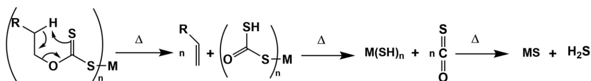
Scheme 1. Xanthate pyrolysis by the Chugaev elimination mechanism 62, 63 .
