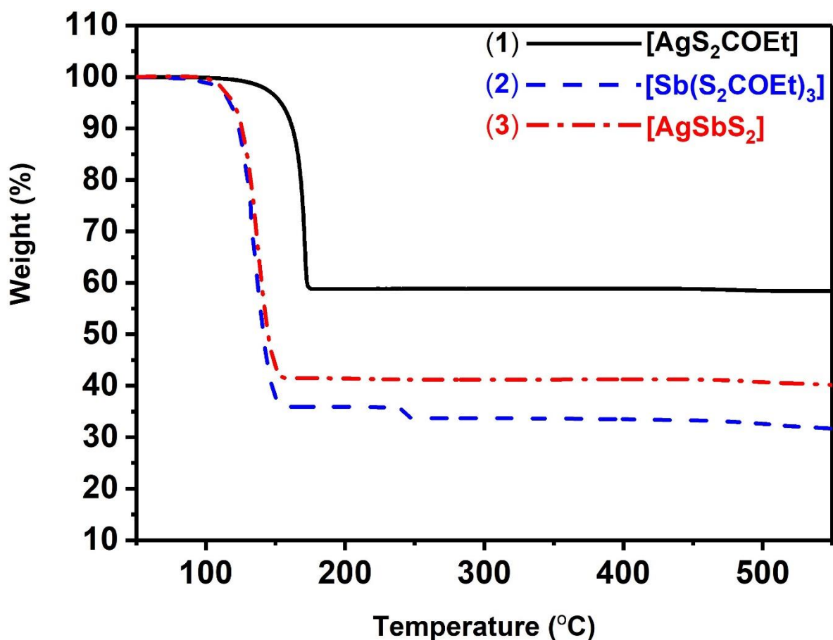
Fig. 2 Thermogravimetric analysis (TGA) of (1) [AgS 2 COEt], (2) [Sb(S 2 COEt) 3 ], and (3) mixtures of Ag and Sb xanthates to form AgSbS 2 .
