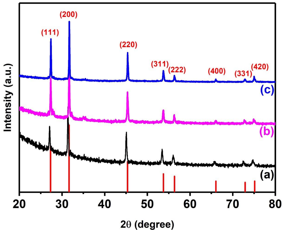
Fig. 3 XRD patterns of \text{AgSbS}_2 powders synthesised at various temperatures (a) 400 °C (b) 450 °C, and (c) 500 °C for 1 h under nitrogen. The red sticks correspond to the standard powder diffraction pattern of cubic \text{AgSbS}_2 (cuboargyrite, ICDD no. 00-017-0456).
