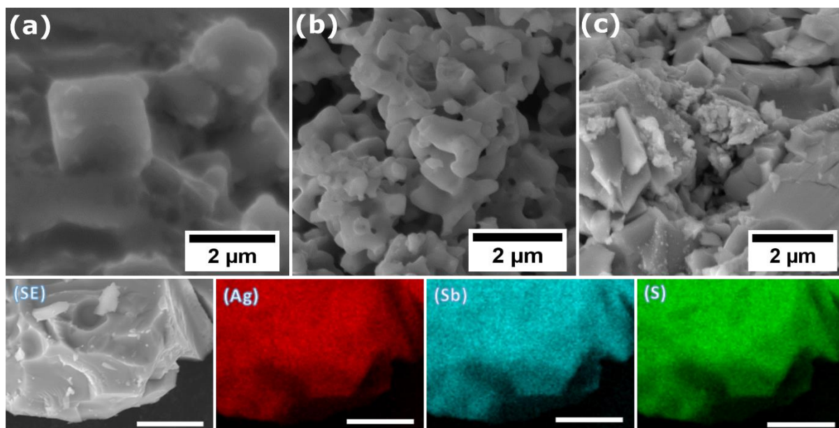
Fig. 6 Top: SEM images of \text{AgSbS}_2 powders produced at (a) 400, (b) 450 and (c) 500 °C, respectively. Bottom: EDX elemental maps revealing the distribution of Ag, Sb and S elements at the microscale for \text{AgSbS}_2 produced at 500 °C (Ag K\alpha , Sb K\alpha and S K\alpha ). The unlabelled scale bars represent 10 \mu\text{m} .
