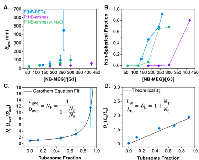
Figure 6. Summary of image analysis data as calculated from acquired dry-state TEM images. (A) Evolution of S_{\text{ave}} values with increasing targeted DP P(\text{NB-MEG}) for P(\text{NB-PEG})_{11} - b - P(\text{NB-MEG})_n (blue circles) and P(\text{NB-amine})_{11} - b - P(\text{NB-MEG})_n diblock copolymer nano-objects developed via aqueous ROMPISA in the absence (purple circles) or presence (green circles) of NaCl. (B) Sample composition, expressed as the fraction of non-spherical nano-objects, as a function of targeted DP P(\text{NB-MEG}) for the same samples. For P(\text{NB-PEG})_{11} - b - P(\text{NB-MEG})_n diblock copolymer nano-objects: C) Evolution of N_F (= L_{\text{ave}}/D_{\text{ave}}) values, the average number of fused particles per tubesome, as a function of the fraction of cylindrical tubesomes in the sample. The black line represents a “step-growth-like” fit of the data using a modified version of Carothers equation ( R^2 = 0.997 ). (D) Evolution of tubesome length dispersity, D_L (= L_w/L_n) values with increasing cylindrical tubesome fraction. The black line represents theoretically expected D_L values calculated from a “step-growth-like” fit of the data using a modified version of Carothers equation ( R^2 = 0.981 ).
