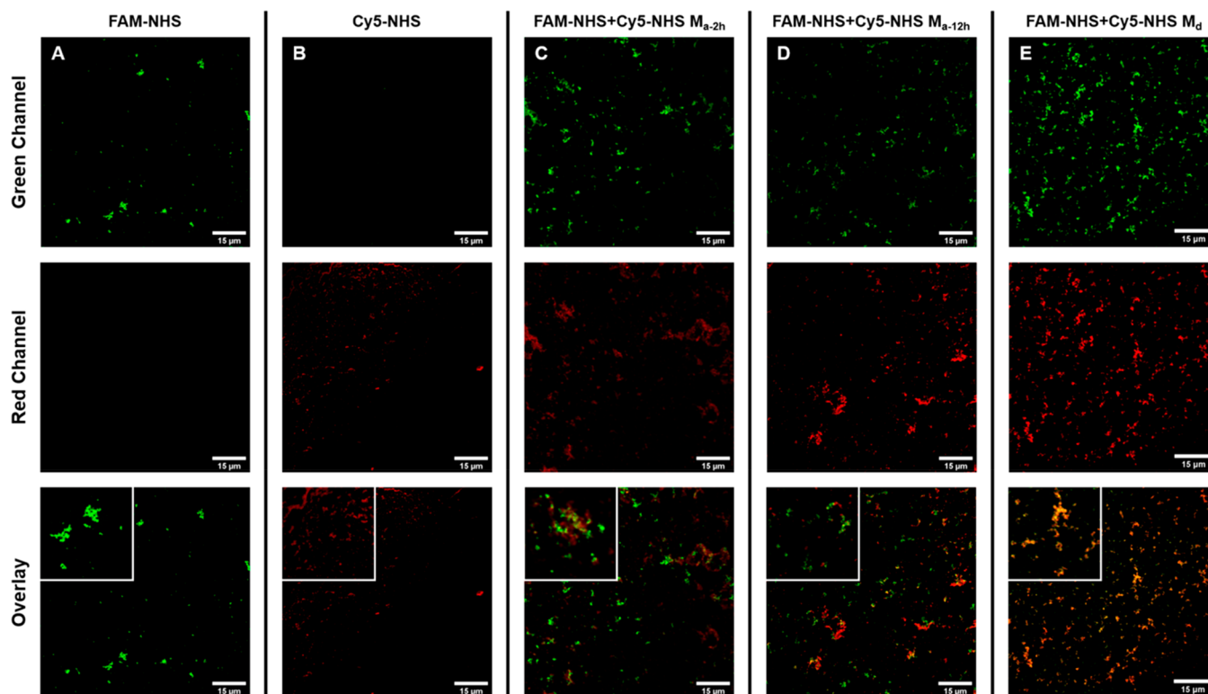
Figure 5. Representative confocal microscopy images for pure FAM-NHS-loaded (green; A) and Cy5-NHS-loaded (red; B) \text{P}(\text{NB-PEG})_{11}\text{-}b\text{-P}(\text{NB-MEG})_{240} diblock copolymer nano-objects, and resulting FAM-NHS+Cy5-NHS M_{a-2h/12h} (C and D) and FAM-NHS+Cy5-NHS M_d (E) samples for investigation of inner aqueous lumen mixing of polymersomes during tubosome development. In all cases, the scale bars represent 15 \mu\text{m} and the size of the insets is 20 \mu\text{m} \times 20 \mu\text{m} .
