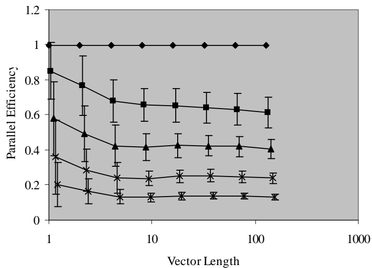
Figure 6.3.8: Parallel AIRS: Parallel Efficiency when Varying the Length of the Input Vector (x-axis offset applied for visual clarity)
