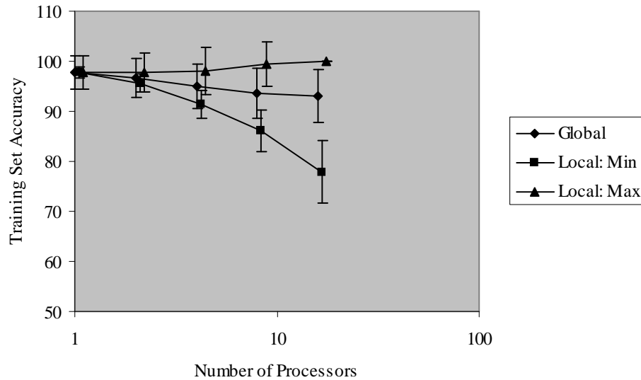
Figure 7.2.12: Distributed AIRS: Sonar: Training Set Accuracies (x-axis offset applied for visual clarity)
