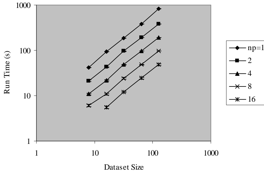
Figure 5.3.1: Parallel CLONALG: Effect of Varying the Number of Input Vectors on Run Time
