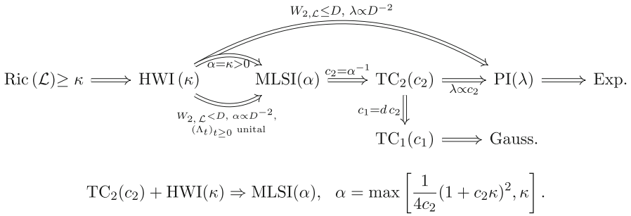
FIGURE 2. Chain of quantum functional- and Talagrand inequalities and related concentrations for a primitive semigroup (\Lambda_t)_{t \geq 0} with generator \mathcal{L} defined on a Hilbert space of dimension d . The implication \text{MLSI}(\alpha) \Rightarrow \text{PI}(\lambda) was proved in [16]. Here, “Exp.” refers to the notion of exponential concentration, whereas “Gauss.” refers to the stronger notion of Gaussian concentration. The implications \text{MLSI}(\alpha) \Rightarrow \text{TC}_2(c_2) \Rightarrow \text{PI}(\lambda) \Rightarrow \text{Exp.} , as well as \text{TC}_2(c_2) \Rightarrow \text{TC}_1(c_1) \Rightarrow \text{Gauss.} were proved in [24]
