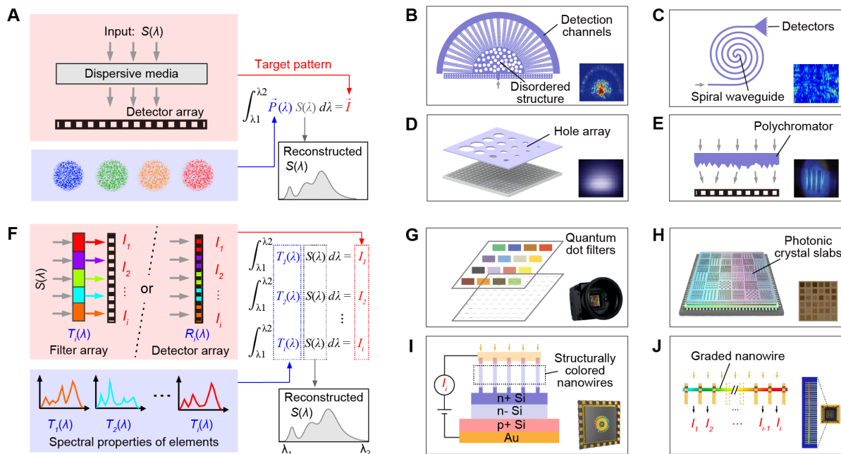
Figure 5. Computational microspectrum systems. (A) Operational principles behind spectrometers based on spectral-to-spatial mapping. (B) – (E) Examples of optical systems that had been adopted for complex spectral-to-spatial mapping: (B) a disordered photonic chip, (C) a spiral waveguide, (D) a dispersive hole array, or (E) a polychromator. [(B) – (E) are adapted with permission from (73, 75-77)]. (F) Principles behind reconstructive spectrometers based on engineered spectral response filtering or detection. (G) – (J) Examples of different reconstructive systems using spectrally-engineered filtering, with arrays based on (G) colloidal quantum dot mixtures and (H) photonic crystal slabs, and spectrally-engineered detection, based on (I) arrays of structurally colored nanowires, and (J) a single, compositionally engineered nanowire. [(G) – (J) are adapted with permission from (78) (80) (86) (13)].
