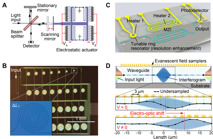
Figure 4. Fourier Transform microspectrometer platforms. (A) Schematic of a miniaturized, MEMS FT spectrometer based on a Michelson interferometer. The path lengths of the interferometer are varied over time via the electrostatic actuator to collect an interferogram which is subsequently converted to spectral data by Fourier transform (56). (B), (C) MZI-based, on-chip Fourier transform spectrometers. (B) Optical image of an SHS device based on an array of multiple MZIs with different OPDs, each varying by \Delta L_i . (C) Schematic of a microspectrometer based on a single MZI, using a micro-ring resonator (MRR) for resolution enhancement and a heater to facilitate path length modulation by thermo-optical effect. [(B) and (C) are adapted with permission from (63, 66).] (D) Schematic (top) of a standing-wave integrated Fourier transform spectrometer system in an electro-optically tunable medium; diagrams (below) illustrate the use of the electro-optic effect in \text{LiNbO}_3 to shift the interferogram along the waveguide over time through application of a bias, V . [(D) is adapted with permission from (71).]
