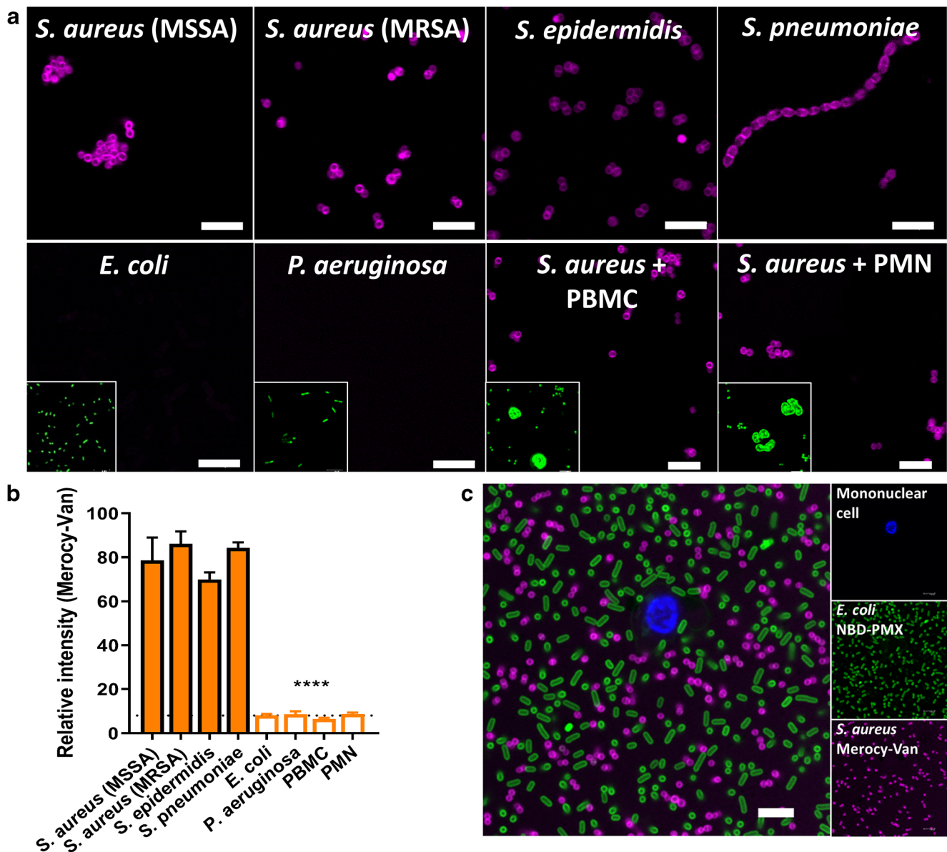
Fig. 2 Merocry-Van selectively labels Gram-positive bacteria. a S. aureus , MRSA, S. epidermidis , S. pneumoniae , E. coli , P. aeruginosa , and S. aureus /mononuclear cell (PBMC) or granulocyte (PMN) co-cultures were imaged by confocal microscopy following the addition of 5 \mu M probe (magenta). Image inserts show counterstained bacteria/cells (green). Representative images from nine fields-of-view from three independent repeats. Scale bar = 5 \mu m. b Quantification of
