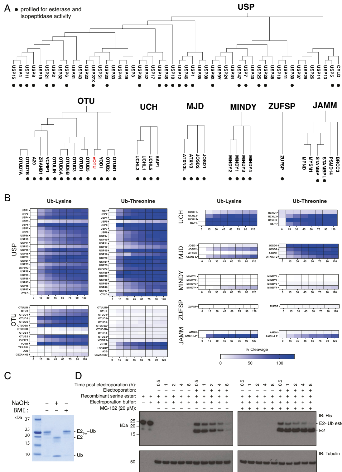
Fig. 2. DUB esterase and isopeptidase screen by MALDI-TOF mass spectrometry and assessment of cellular ubiquitin ester stability. (A) Phylogenetic classification of deubiquitinating enzymes based on their catalytic domains. Only DUBs that are active and recognize ubiquitin are displayed. The vOTU (red) catalytic domain exists within Protein L, which is encoded by Crimean-Congo hemorrhagic fever virus. DUBs annotated with a solid circle correspond to those profiled for activity in this study. (B) A panel of 53 DUBs were tested for their activity toward model substrates Ub-Lys and Ub-Thr. Reactions were then quenched by addition of TFA (2%) at the relevant time points and spotted onto a 1536 AnchorChip target plate, followed by MALDI-TOF analysis (17). Results are reported as percent of cleavage in a scale from white (no activity) to dark blue (100% substrate consumption). Employed DUB concentrations are specified in SI Appendix, Table S1 . (C) An engineered E2~Ub conjugate linked to the Ub C terminus via a serine ester (E2 ser ~Ub) was used as model ester-linked substrate. Resistance to BME, but sensitivity to NaOH, is consistent with the conjugate being ester-linked. (D) E2 ser ~Ub was delivered into HEK293 cells by electroporation and then transferred directly into prewarmed media and then incubated at 37 °C, 5% CO 2 . Samples were taken at the indicated time points postelectroporation. The experiment was replicated in parallel, using HEK293 pretreated with 20 μM MG132 for 30 min, and cells incubated in media containing MG-132 throughout.
