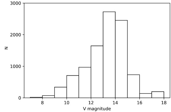
Figure 8. The distribution of NOMAD V magnitude of SVS stars with a variable-type classification and correct period classification ranges between 8 \geq V \geq 18 .
