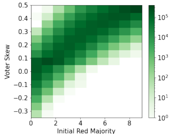
Figure 6: Histogram of initial majority and final voter skew for homophilic relaxed-caveman graphs generated by dataset 2. Colours denote the frequency of each bin. Having a Pearson correlation of \rho = 0.904 , majority predicts the election outcome better than IG.
