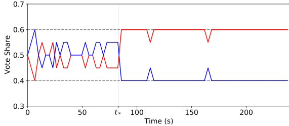
Figure 3: Example time series of a voting game, using Stewart et al. [43] behavioural model on a homophilic relaxed-caveman graph with rewire parameter p_0 = 0.3 and homophily h = 0.3 . The two parties initially have equal vote share but eventually the red party reaches a super-majority of V = 0.6 (the dashed lines are V and 1 - V ). The vertical dotted line at t_* represents the transition between early and late phases of the game.
