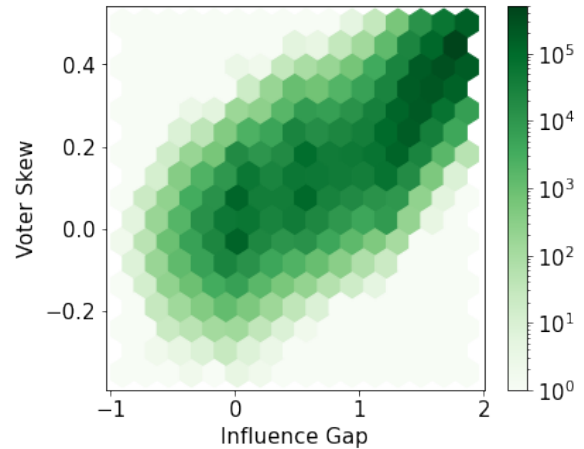
Figure 5: Histogram of influence gap and final voter skew for homophilic relaxed-caveman graphs generated by dataset 2. Colours denote the frequency of each bin. The relationship is statistically strong, with Pearson correlation of \rho = 0.891 .
