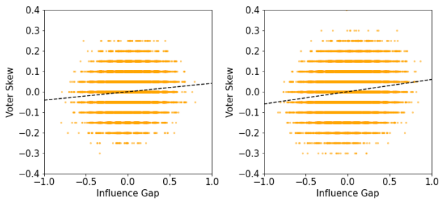
Figure 4: Simulations of the behavioural model of Stewart et al. [43] acting on relaxed- and homophilic relaxed-caveman graph for dataset 1. In both cases the influence gap correlates very weakly with voter skew, having a Pearson’s \rho < 0.2 , and passing a significance test with p < 10^{-5} . Left: for the relaxed-caveman graph with rewiring parameter p = 0.3 gives rise to a Pearson correlation of \rho = 0.104 . Right: for the homophilic relaxed-caveman with rewiring probability p_0 = 1 and homophily factor h = 0.3 the correlation is slightly more pronounced with \rho = 0.160 .
