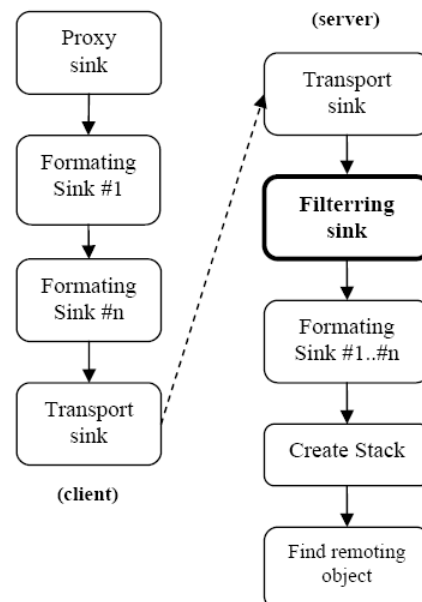
Fig. 4. Traffic filtering
