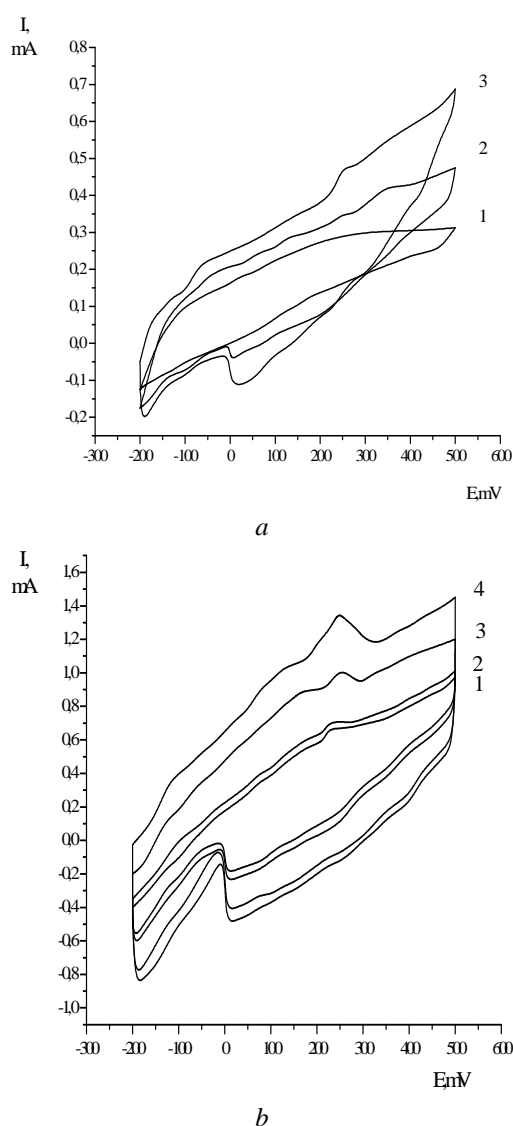
Fig. 2. Voltammograms of CNT electrode in solutions with different content of mercury; (a): 1 – supporting electrolyte; 2 – 0.02; 3 – 0.04 \text{mcg}\cdot\text{dm}^{-3} ; (b): 1 – 0.1; 2 – 0.5; 3 – 1; 4 – 2 \text{mcg}\cdot\text{dm}^{-3}
