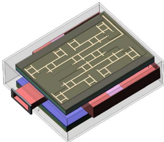
Fig.2. Strip line RF power adder
