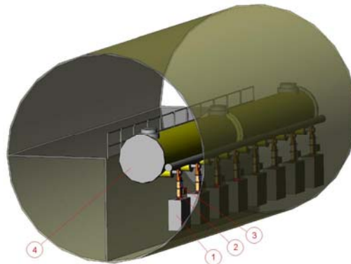
Fig. 5. Accelerator module with Solid State High Power RF System in XFEL tunnel.
