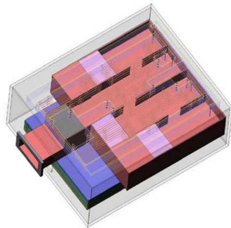
Fig.3. Waveguide RF power adder
