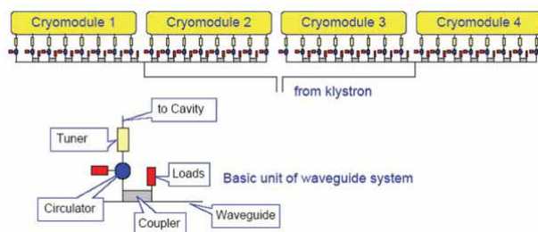
Fig.1. RF waveguide distribution of klystron based XFEL RF station
