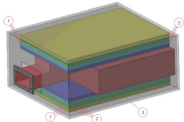
Fig.4. General view of Solid State Generator 1 is amplifier unit, 2 is strip line RF power adder, 3 is waveguide RF power adder
