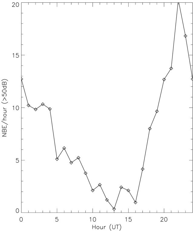
NPM to SGO: Diurnal variation
