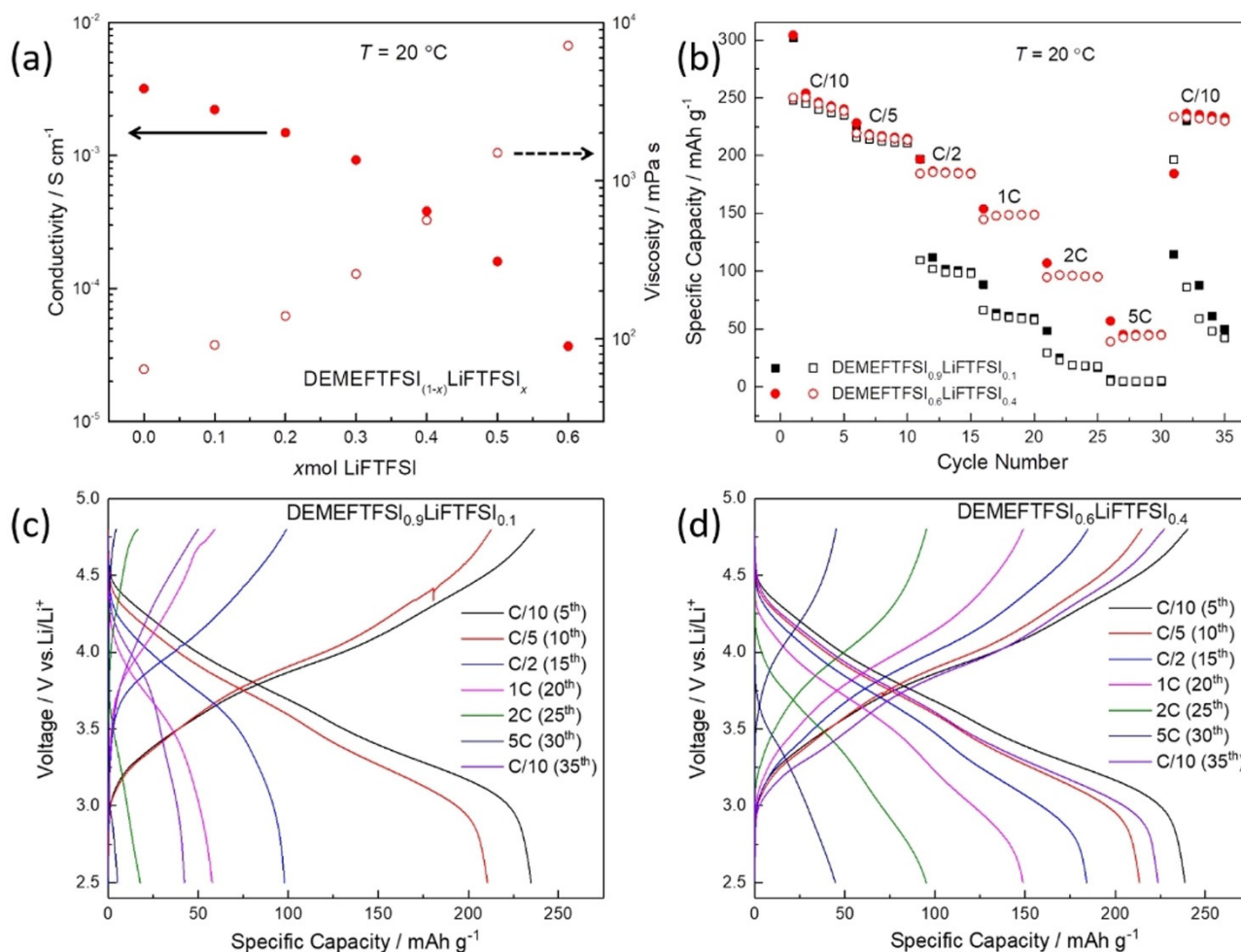
Figure 4. (a) Isothermal conductivity and viscosity of DEMEFTFSI _{(1-x)} LiFTFSI _x . (b) Rate performance in the voltage range of 2.5–4.8 V and selected voltage profiles of Li/DEMEFTFSI _{(1-x)} LiFTFSI _x /LMR cells with x = 0.1 (c) and 0.4 (d).
