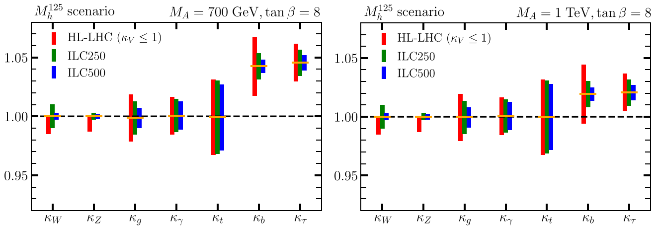
Fig. 9 Wäscheleinen-plots for the two assumed MSSM parameter points (M_A, \tan \beta) = (700 \text{ GeV}, 8) (left) and (M_A, \tan \beta) = (1 \text{ TeV}, 8) (right) in the M_h^{125} scenario: Predicted Higgs couplings in the \kappa framework (orange horizontal bars) along with the anticipated
