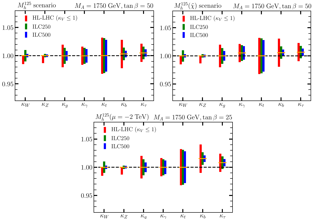
Fig. 15 Wäscheleinen-plots, using the same color coding as in Fig. 9, for the following three assumed MSSM scenarios: (M_A, \tan \beta) = (1750 \text{ GeV}, 50) in the M_h^{125} scenario (upper left panel), (M_A, \tan \beta) = (1750 \text{ GeV}, 50) in the M_h^{125}(\tilde{\chi}) scenario (upper right), and (M_A, \tan \beta) = (1750 \text{ GeV}, 25) in the M_h^{125,\mu^-} scenario (lower panel).
