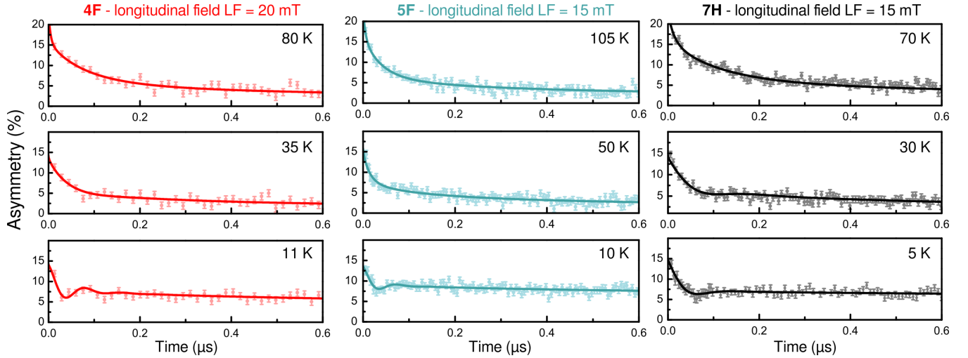
FIG. 3. From left to right: muon asymmetry data for 4F (LF = 20 mT), and 5F and 7H (LF = 15 mT) collected at different temperatures. Solid lines are best fit curves (see text).
