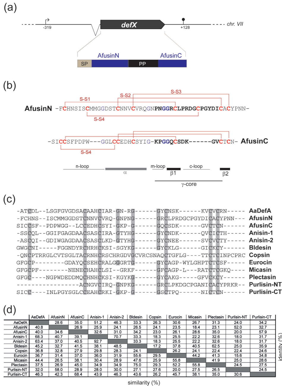
FIGURE 1 The defX gene of A. fumigatus has the capacity to encode two CS \alpha \beta defensin-like peptides. (a) Schematic overview on the annotated defX gene locus on chromosome VII of the A. fumigatus genome (AfuA_7G05180), with positions of transcriptional initiation and termination indicated relative to the start and stop codon, respectively, of the coding sequence. The deduced gene product comprises a signal peptide (SP) and two defensin-like peptides, AfusinN and AfusinC that are processed from the primary translation product after removal of a pro-peptide (PP) spacer region. (b) Sequence and connectivity between conserved cysteines of the deduced CS \alpha \beta -defensin-like peptides. Cysteine residues forming disulfide bridges are highlighted in red, conserved glycine residues in blue, and structural elements are illustrated below with corresponding residues of the \gamma -core segment in bold. (c) Global alignment of selected fungal defensin-like peptides and the originating insect defensin AaDefA of the mosquito Aedes aegypti , with conserved (>50%) residues – the disulfide bridging cysteines and two glycine residues – highlighted in grey. Aligned peptides with sequence identifiers are AaDefA of A. aegypti (ASY93145), AfusinN and AfusinC of A. fumigatus (XP_748991), Anisin-1 and Anisin-2 of A. nidulans (XP_662650 and CBF69423), Bldesin of Blastomyces dermatitidis (EQL35841), Copsin of Coprinopsis cinerea (AIU55999), Eurocin of Eurotium amstelodami (K7N5L0), Micasin of Microsporium canis (AEM44801), Plectasin of Pseudoplectanania nigrella (Q53106), and Purlisin-NT and Purlisin-CT of Purpureocillium lilacinum (PWI75532). (d) Tabular overview on similarities and identities between above selected fungal DLPs as deduced from pairwise global alignments (Needleman-Wunsch algorithm)
