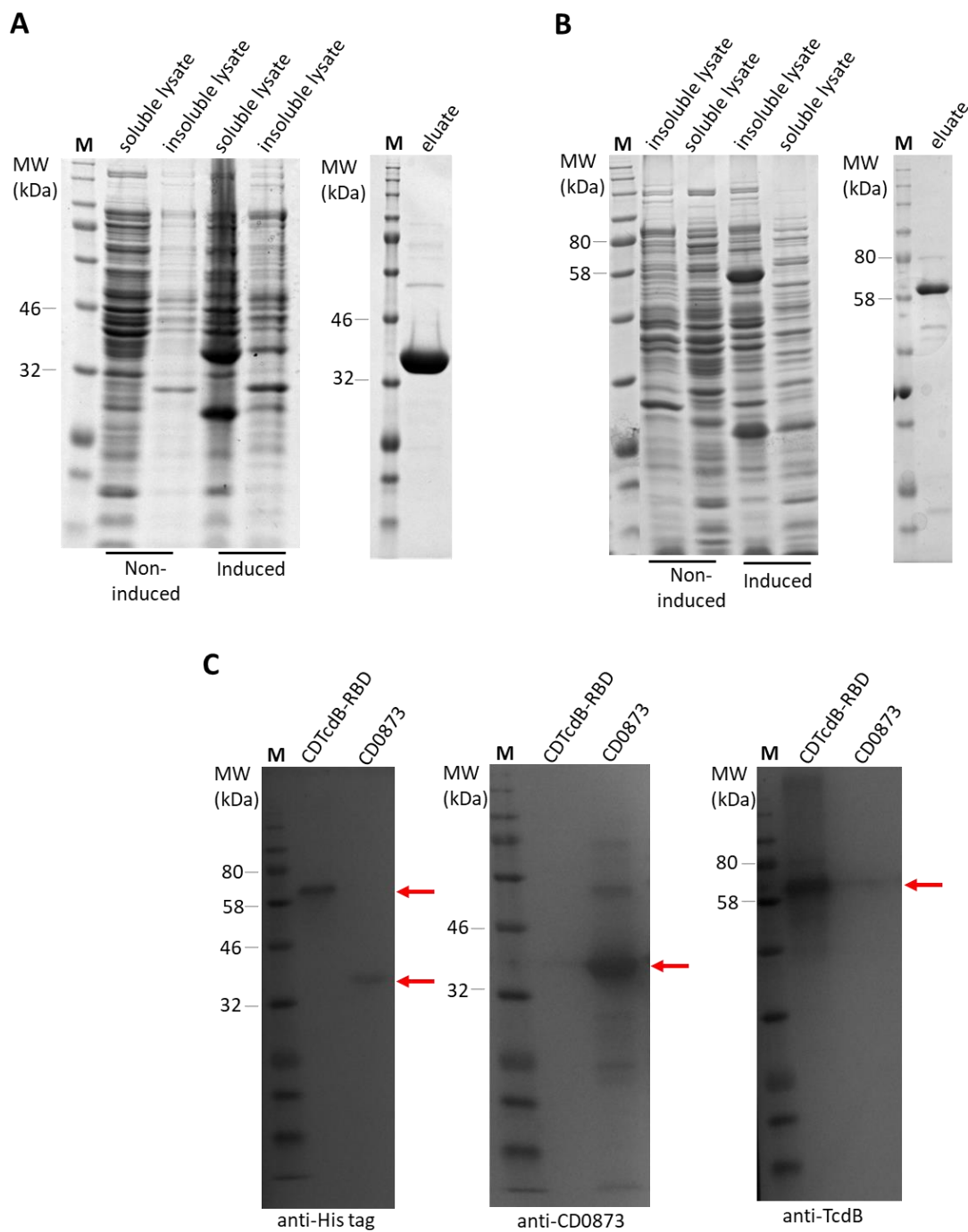
Figure 2. Purification of recombinant protein antigens. Protein extracts of soluble and insoluble fractions from induced and non-induced cultures of recombinant E. coli strain T7 and the eluates obtained after IMAC were separated by SDS-PAGE (10% acrylamide) and stained by Coomassie Blue ( A,B ) or analysed by Western immunoblotting ( C ). ( A ) Identification of CD0873 in the soluble fraction, ( B ) Identification of CDTcdB-RBD in the insoluble fraction, ( C ) Western immunoblot of purified recombinant CD0873 and CDTcdB-RBD probed with anti-His tag antibody, anti-CD0873 antibody or anti-TcdB antibody and detected by the addition of the appropriate HRP-conjugated secondary antibody and TMB substrate. Lane M: Colour pre-stained protein standard. Bands of expected molecular weight of 36 kDa for CD0873 and 61 kDa for CDTcdB-RBD were detected as indicated by the red arrows.
