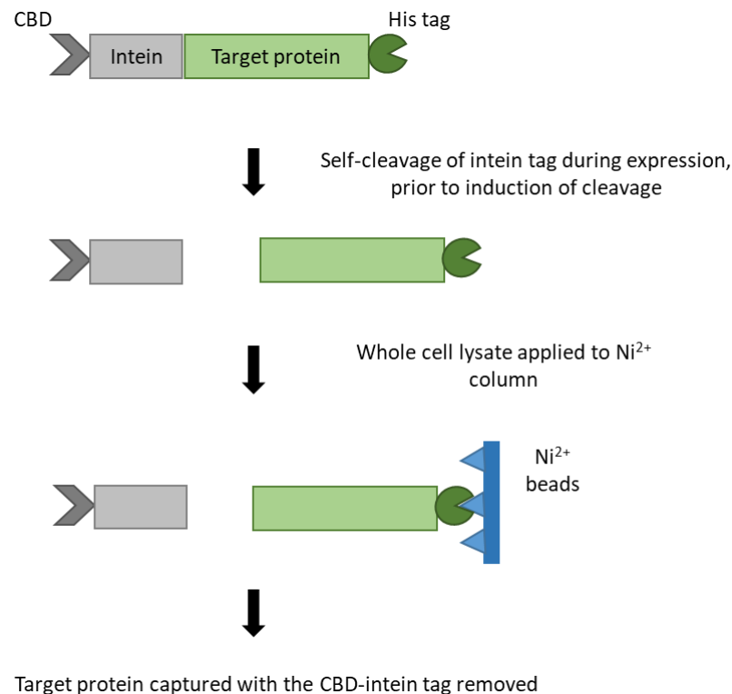
Figure 1. Schematic diagram of pTWIN1-His expression system. The expression vector pTWIN1 (NEB) was modified by the inclusion of a His tag for C-terminal tagging. This prevented loss of the target protein due to excessive natural self-cleavage of the N-terminal intein tag bearing the chitin-binding domain (CBD) by trapping the target protein with a Ni 2+ column by Immobilised Metal Affinity Chromatography (IMAC).
