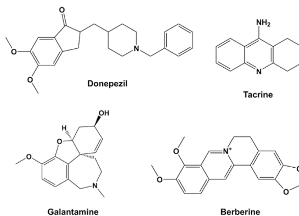
Figure 1. Structures of the cholinesterase inhibitor (ChEI) drugs.
