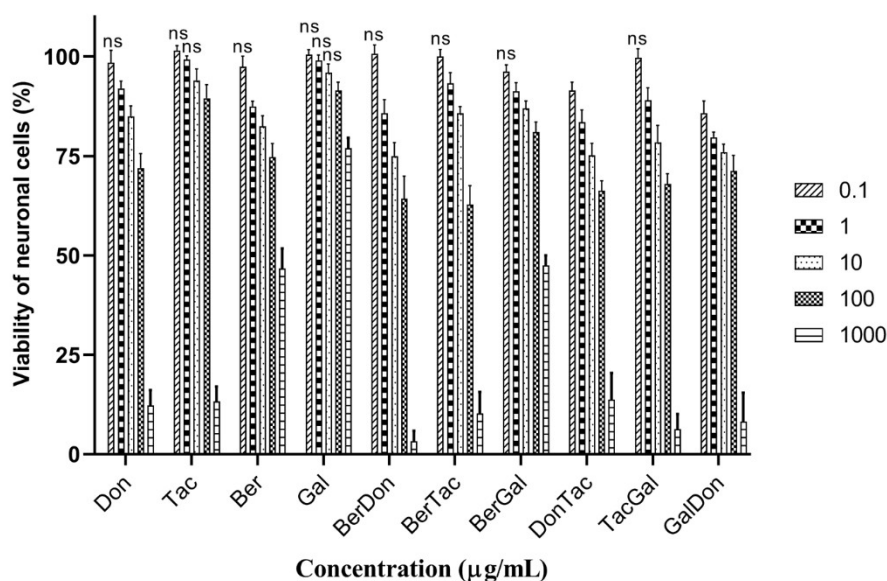
Figure 5. Cytotoxicity of individual and dual-drug ChEI combinations to SH-SY5Y cells: Human neuroblastoma cells were incubated with donepezil (Don), tacrine (Tac), berberine (Ber), and galantamine (Gal) or dual-drug combinations: BerTac (berberine and tacrine), BerGal (berberine and galantamine), TacDon (tacrine and donepezil), DonGal (donepezil and galantamine), DonBer (donepezil and berberine), and TacGal (tacrine and galantamine), and cell viability quantified using a MTT assay. Significant changes were quantified using a one-way ANOVA. ns = non-significant effect on cell viability. All other histograms not marked with ns, displayed significant changes from controls.
