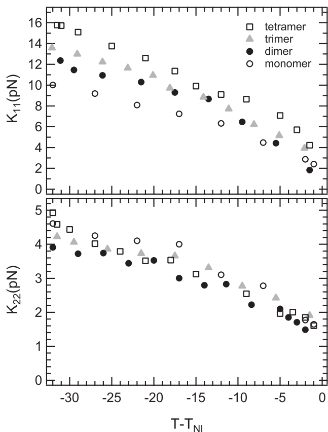
Fig. 6 Splay ( K_{11} , top panel) and twist ( K_{22} , bottom panel) elastic constants plotted as a function of temperature relative to the nematic-isotropic transition for the studied n-mers.
