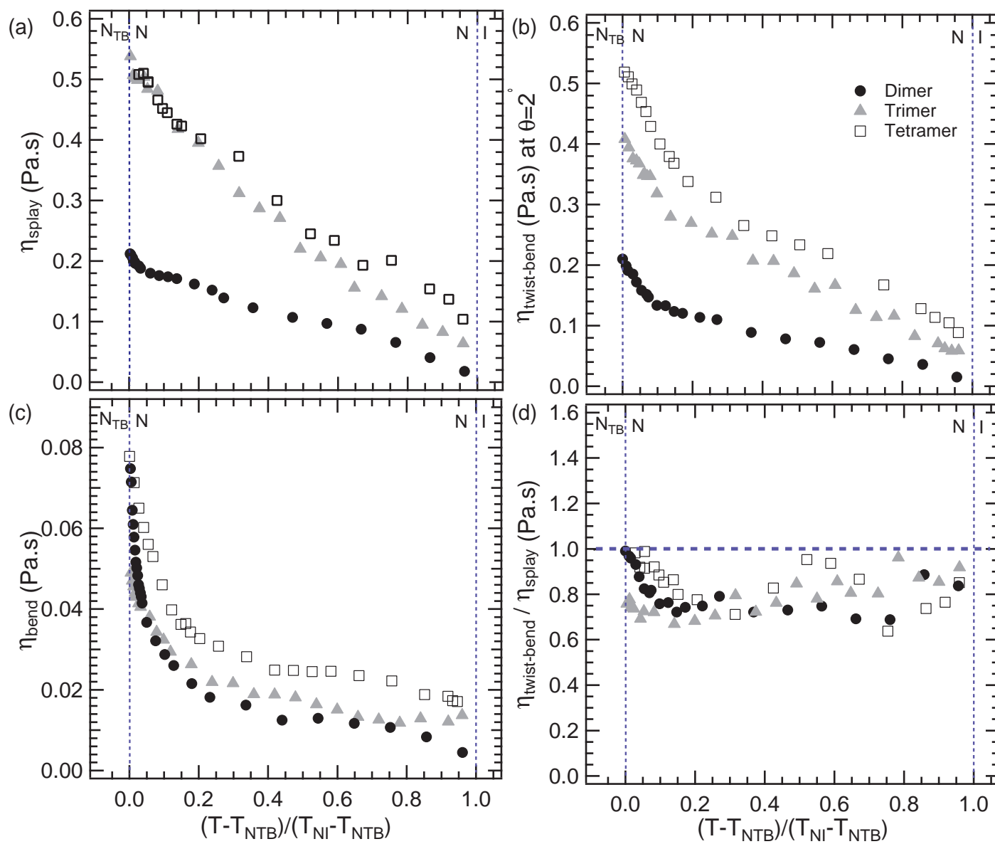
Fig. 4 Reduced temperature dependences of the nematic orientational viscosities in the studied n-mers. (a) – (c): \eta_{splay} , \eta_{twist-bend} , and \eta_{bend} ; (d): The ratio \eta_{twist-bend} / \eta_{splay} .
