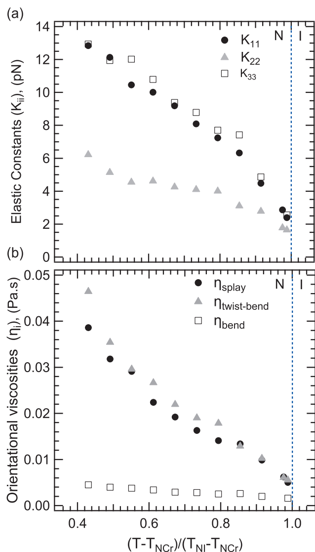
Fig. 5 Elastic constants (a) and viscosities (b) as a function of reduced temperature in the N phase of the monomer MCT5. T_{NCr} is the temperature of the nematic to crystal transition.
