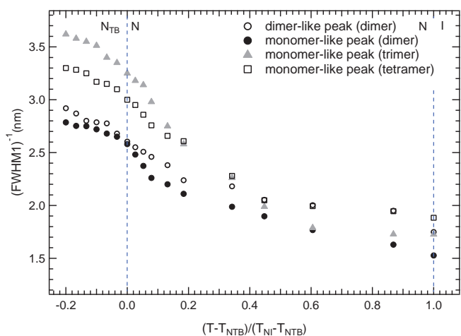
Fig. 7 Inverse full width at half maximum of the “monomer”-like peak, recorded by small-angle X-ray scattering (SAXS) from the studied n-mers, and of the “dimer”-like peak, recorded on the dimer. Data are plotted for reduced temperatures through the N and into the N_{TB} phase. Here “monomer”- and “dimer”-like refer to diffuse peak positions corresponding to approximately the length of the monomer unit and to approximately twice this length. The values of (FWHM)^{-1} were obtained from fitting the azimuthally averaged SAXS profiles to a sum of Lorentzians.
