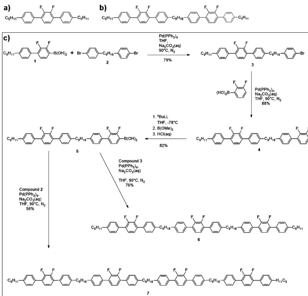
Fig. 1 a) and b): Molecular structures of MCT5 monomer and DTC5C9 dimer. c): Synthetic scheme for the homologous trimer 6 and tetramer 7 .
