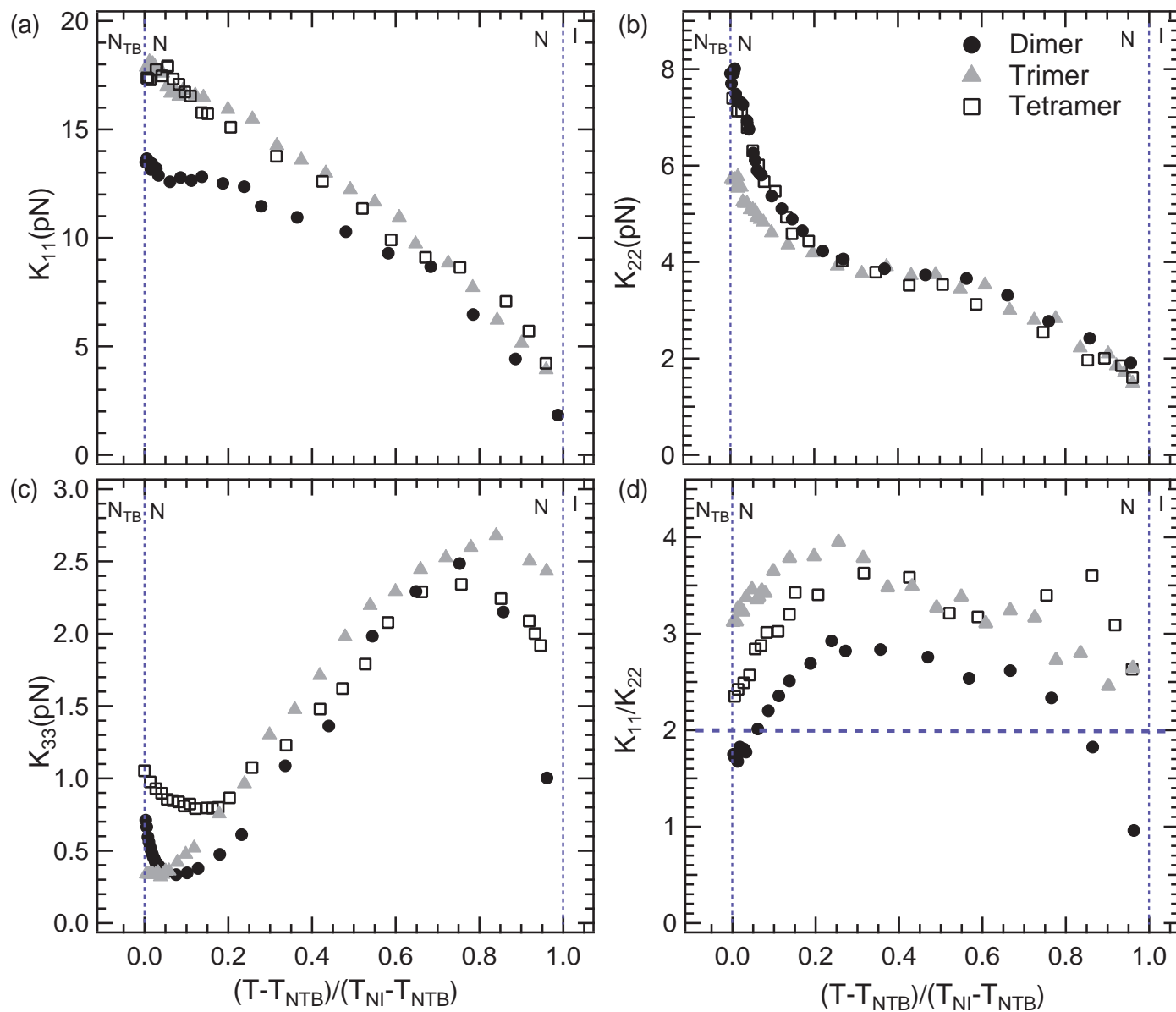
Fig. 3 Reduced temperature dependences of the nematic elastic constants. (a) – (c): Splay ( K_{11} ), twist ( K_{22} ), and bend ( K_{33} ) constants for the dimer, trimer, and tetramer; (d): The ratio K_{11}/K_{22} with the theoretical threshold value for a N_{TB} phase indicated by a horizontal dashed line.
