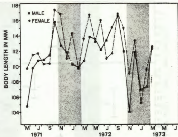
FIG. 3. Average body length measurements of ♂ and ♀ prairie voles by month. Body length equals total length minus tail length. Winter months are shaded.
