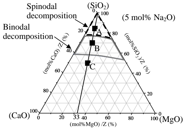
Figure 1. Calculated composition ranges for spinodal decomposition and binodal decomposition for the SiO 2 -CaO-MgO-5 mol% Na 2 O system at 948 K. (Z= mol% (SiO 2 +CaO+MgO))
