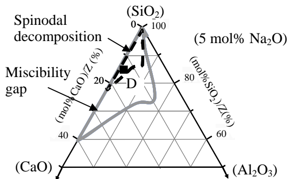
Figure 3. Calculated metastable immiscibility regions including spinodal decomposition in the SiO 2 -CaO-Al 2 O 3 -5 mol% Na 2 O system at 973 K. (Z= mol% (SiO 2 +CaO+Al 2 O 3 ))
