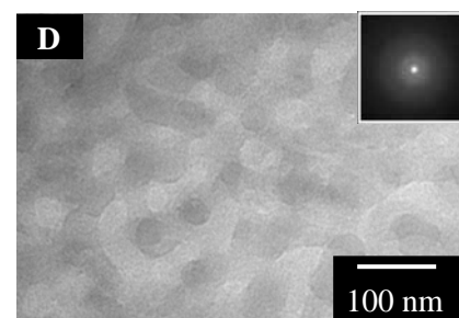
Figure 4. Electron micrograph of glass D (80.8SiO 2 -11.7CaO-2.5Al 2 O 3 -5.0 mol% Na 2 O) annealed for 96 h at 993 K.
