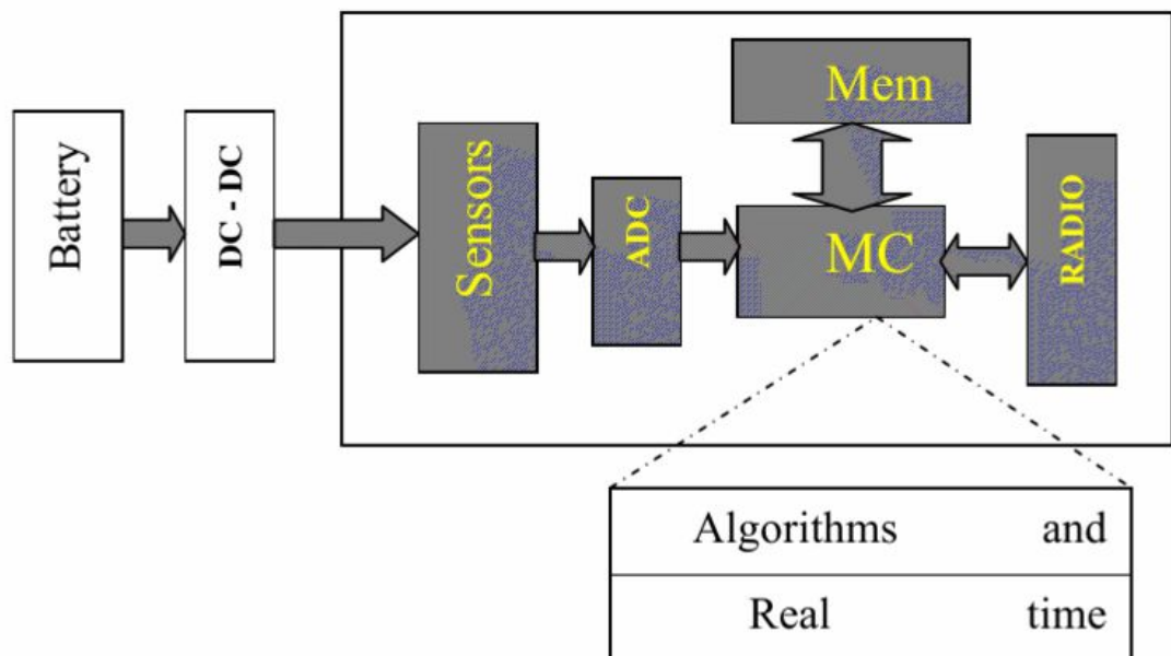
Figure 15. Architecture of a Sensor Node [25]
