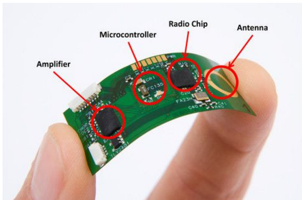
Figure 8. Wireless ECG Sensor with a functional Microcontroller [35]
