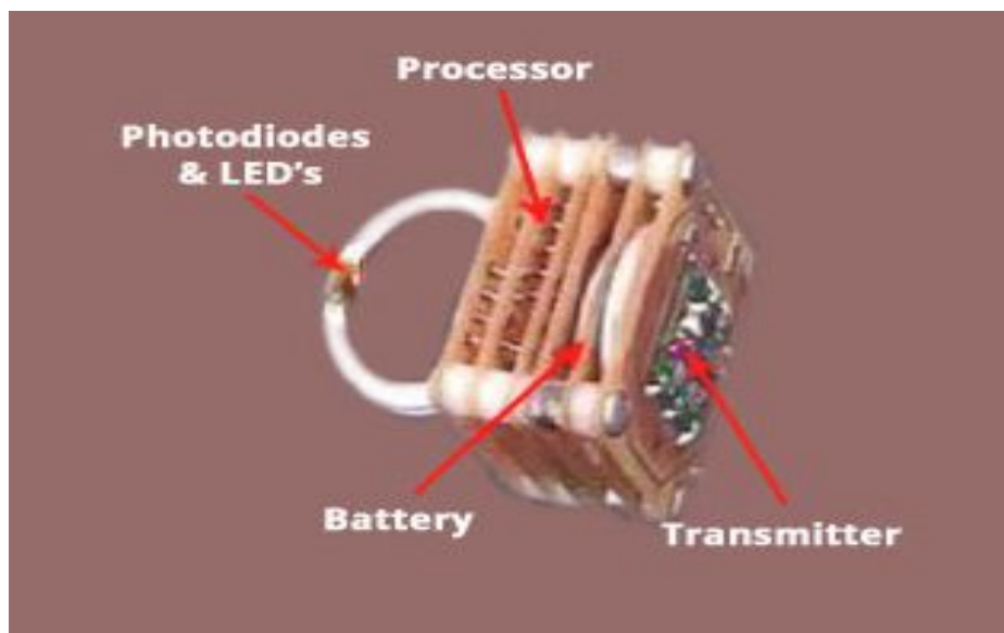
Figure 17. Architecture for Pulse Oximetry Ring.Reprinted [35]
