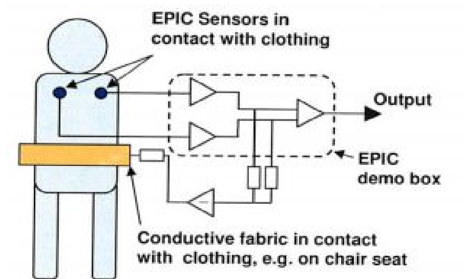
Figure 6. Basic configuration of non-contact ECG sensor [36]
