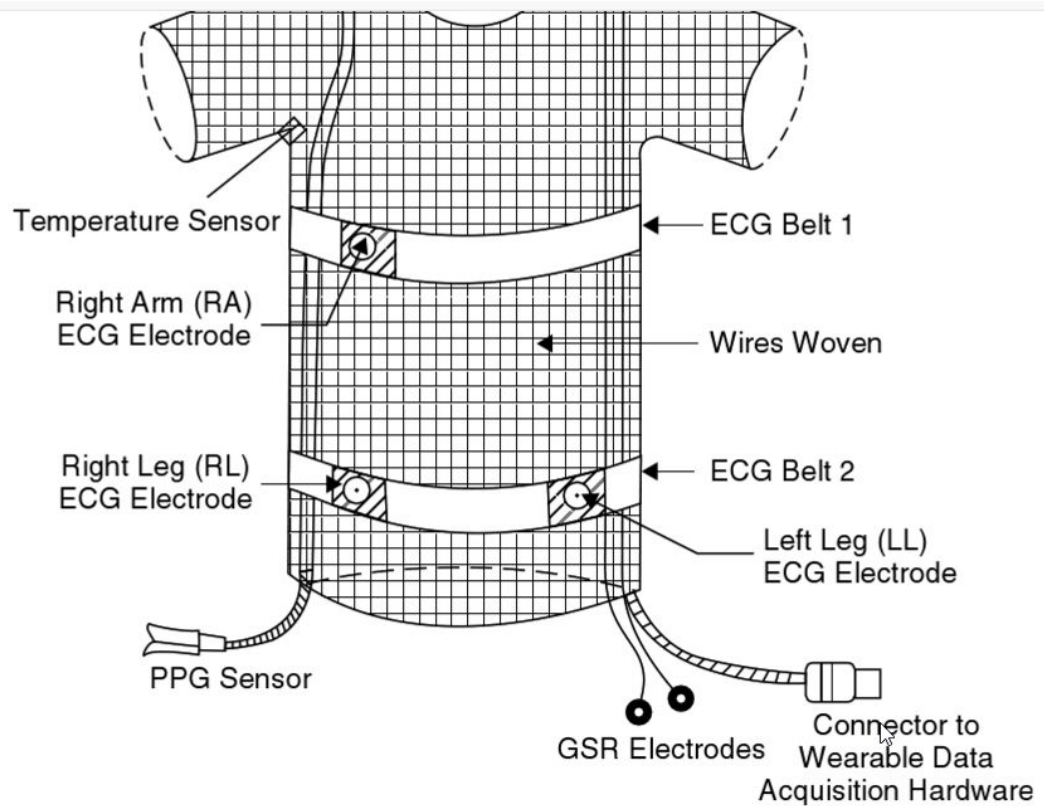
Figure 13. Diagram of a smart vest [4]
