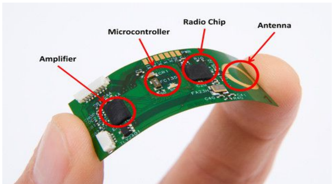
Figure 5. ECG sensor electronics [29]
