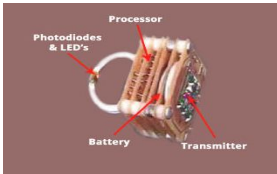
Figure 12. Pulse oximetry ring sensor [35]
