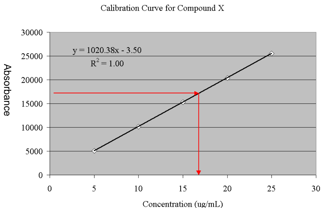
Graph 1 Calibration curve of AAS for an ion (George Mason University, 1998)
