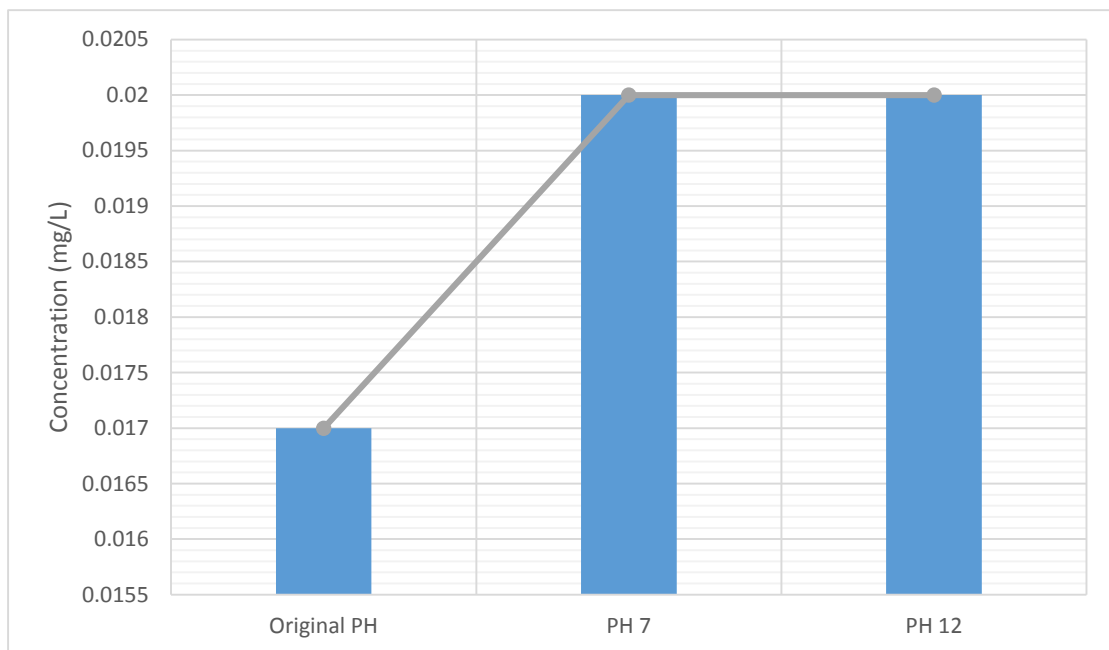
Graph 17. The solubility diagram of aluminum hydroxide (Phifer, M.A., 2000).
