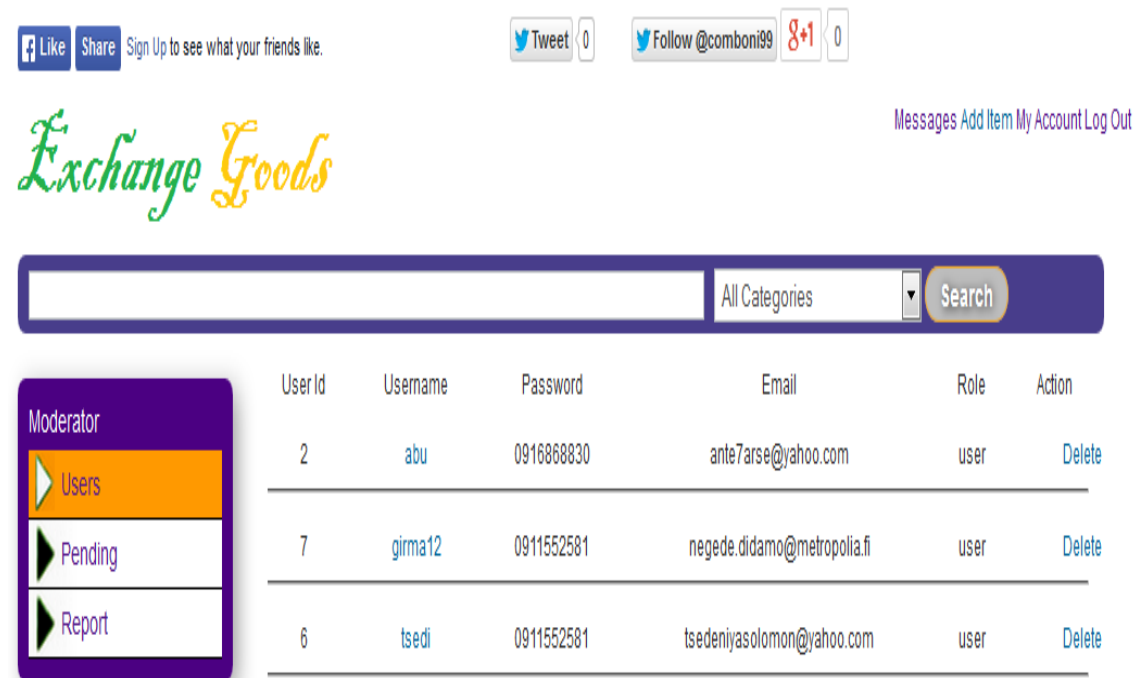
Figure 9. Admin page.
