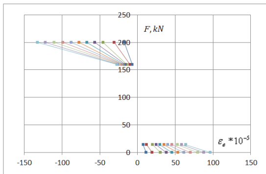
Figure 8. Diagrams of strain distribution in height of normal cross section of samples
