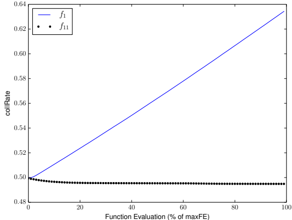
Fig. 2. collRate Changes of f_1 and f_{11}
