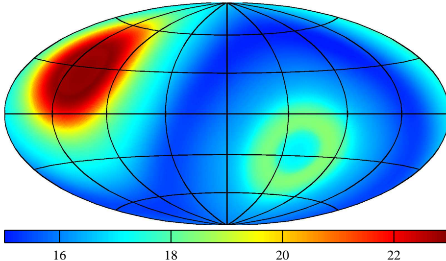
Fig. 1.— The exposure at 1 GeV in Galactic coordinates and Hammer-Aitoff projection for the four-year period analyzed for the 3FGL catalog. The units are equivalent on-axis observing time (in Ms).
