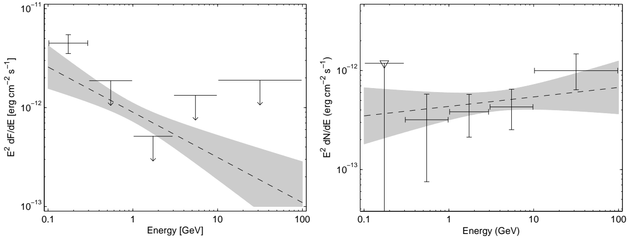
Fig. 7.— Spectral energy distribution of the same source (the BL Lac TXS 0836+182) as 2FGL J0839.4+1802 (left) and 3FGL J0839.6+1803 (right). This source was flagged as ‘possibly due to the Sun’ (Flag 11 in Table 3) in 2FGL. Entering the Sun and Moon into the background model has reduced to zero the low energy signal that drove the 2FGL fit, resulting in a hard source in 3FGL. The dashed line is the best fit over the full energy range (§ 3.2) and the gray-shaded area is the statistical uncertainty around the best fit (for a given spectral form). The vertical scale is not the same in the left and right plots. Note that the 300 MeV to 1 GeV point has (asymmetric) error bars in 3FGL as explained in § 3.5 even though its significance is less than 2\sigma . Upper limits (indicated by a downward triangle in 3FGL and a downward arrow in 2FGL) are at 95% confidence level.
