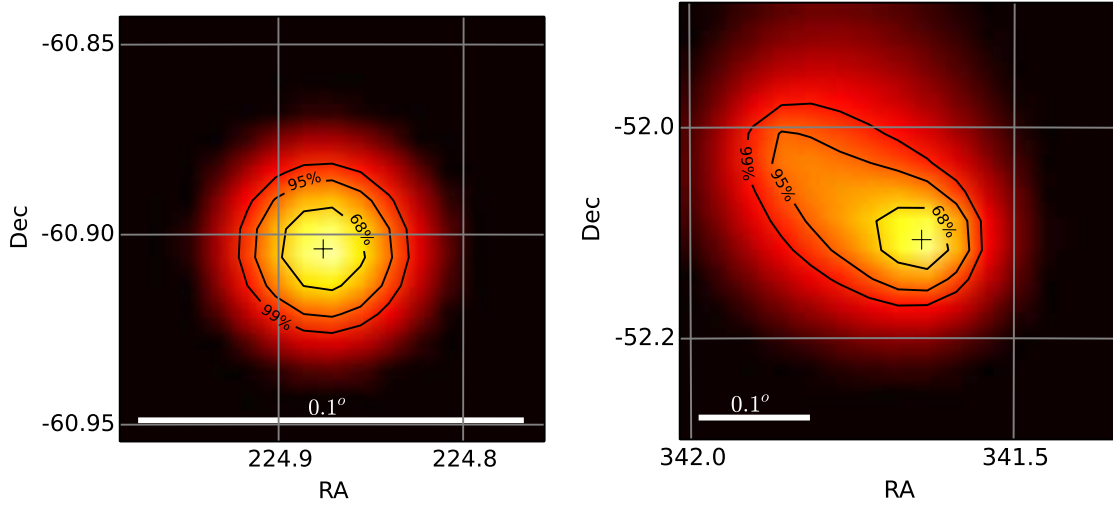
Fig. 5.— Examples of localization TS maps. The contours for 68%, 95%, and 99% containment are shown. The scale (in decimal degrees) is not the same in both plots. Left: PSR J1459–6053, a good localization with LQ = 0.63 . Right: 3FGL J2246.7–5205, a bad localization with LQ = 14 .
