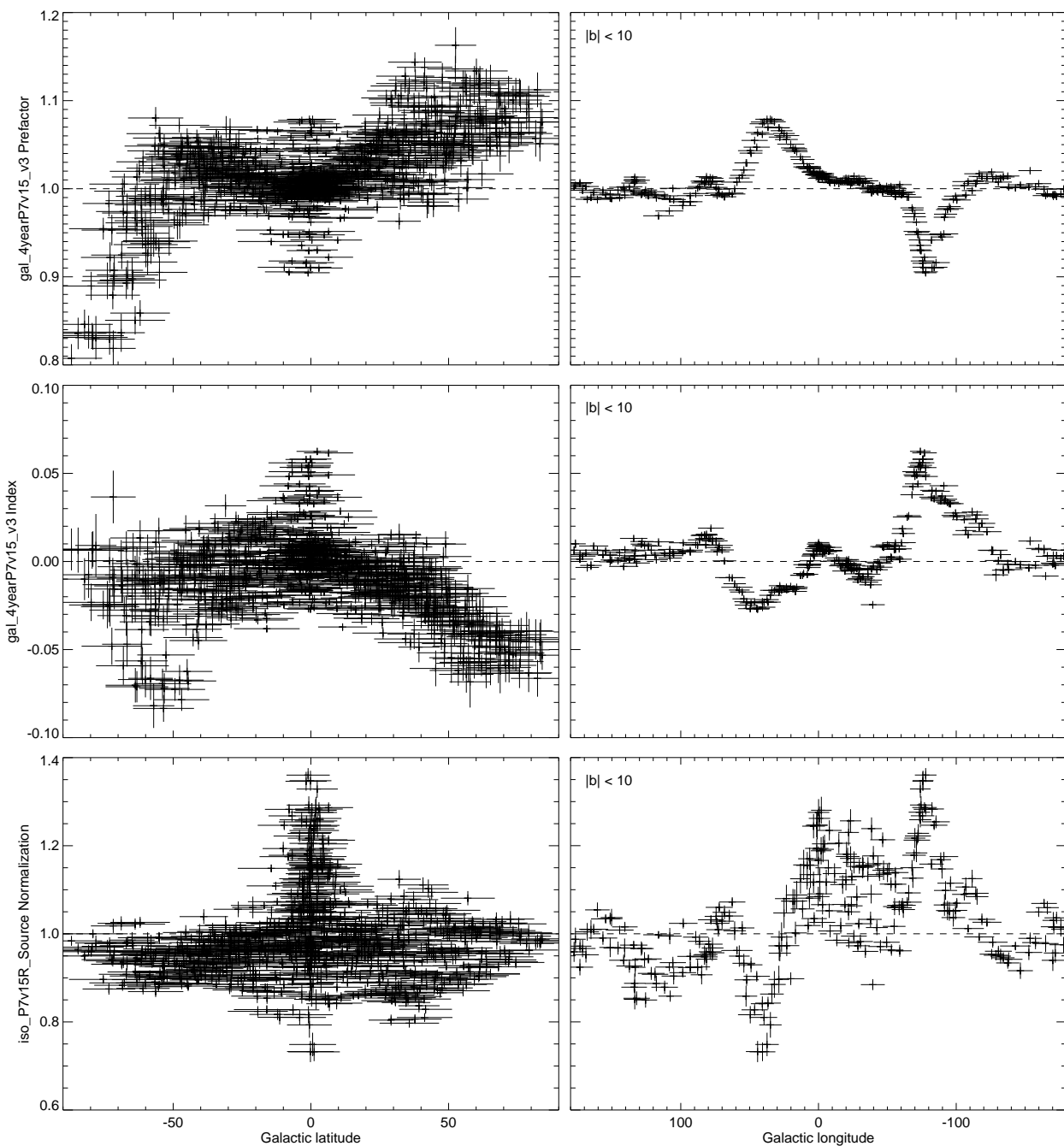
Fig. 25.— Diffuse model parameters in each RoI. The horizontal error bar is the RoI radius. The vertical error bar is the statistical error from the fit. The vertical scale is the same in the left and right plots for a given parameter. Top: Normalization of the Galactic diffuse component (at 500 MeV). Center: Spectral index of the power-law correction to the Galactic diffuse component (positive means a harder model). Bottom: Normalization of the isotropic component. Left: All values as a function of Galactic latitude. Right: Galactic plane only as a function of Galactic longitude.
