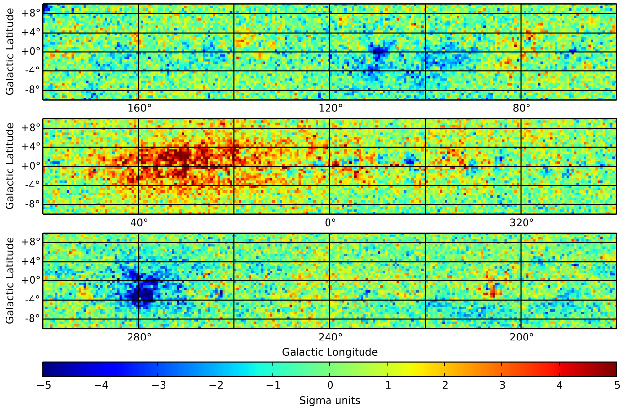
Fig. 26.— Residuals when setting the diffuse model normalizations to 1 and no power-law correction, integrated from 100 MeV to 100 GeV and expressed in sigma units over 0.5^\circ pixels. Top: Positive Galactic longitudes from the anticenter to Cygnus. Center: Galactic ridge. Bottom: Negative Galactic longitudes from Carina to the anticenter.
