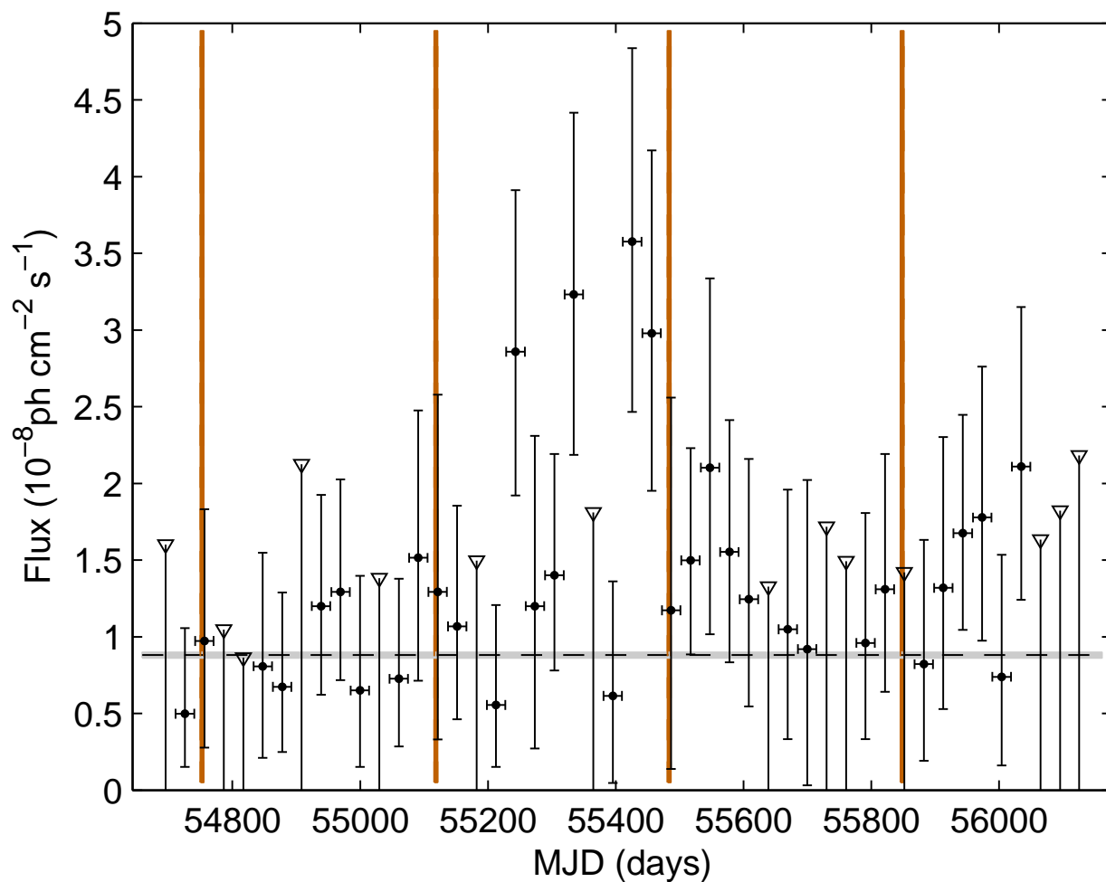
Fig. 10.— Light curve of 3FGL J1315.7–0732 (NVSS J131552–073301) in the ecliptic plane. That source is significantly variable. The flares do not correspond to the times when the Sun passed through the region (vertical orange bands). The only effect of the Sun passage is somewhat larger error bars. The gray-shaded horizontal area materializes the systematic uncertainty of 2%. Upper limits (indicated by a downward triangle) are at 95% confidence level.
