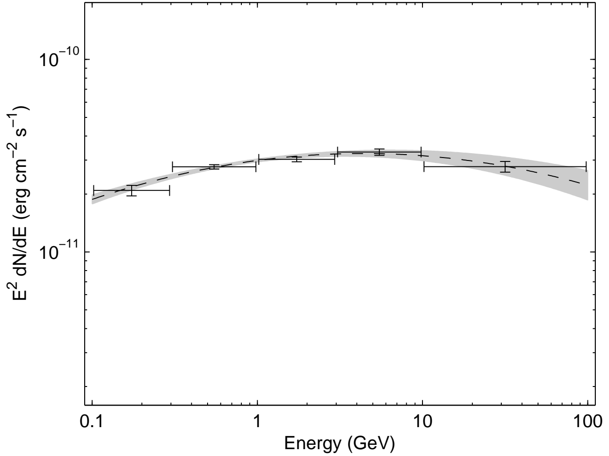
Fig. 8.— Spectral energy distribution of 3FGL J0222.6+4301 (3C 66A) fitted by a LogParabola spectrum with \beta = 0.039 \pm 0.007 but Signif_Curve (defined just before Eq. 3) = 2.81. The curvature is statistically significant but a power law cannot be excluded given the range of the systematic errors on effective area.
