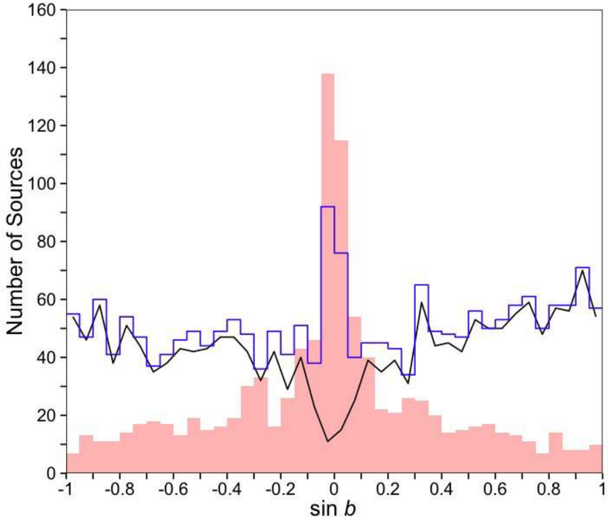
Fig. 23.— Distributions in Galactic latitude b of unassociated sources (shaded red region), all associated sources (blue histogram) and all active galaxy source classes (black line). Binned in \sin b , an isotropic distribution would be flat.
