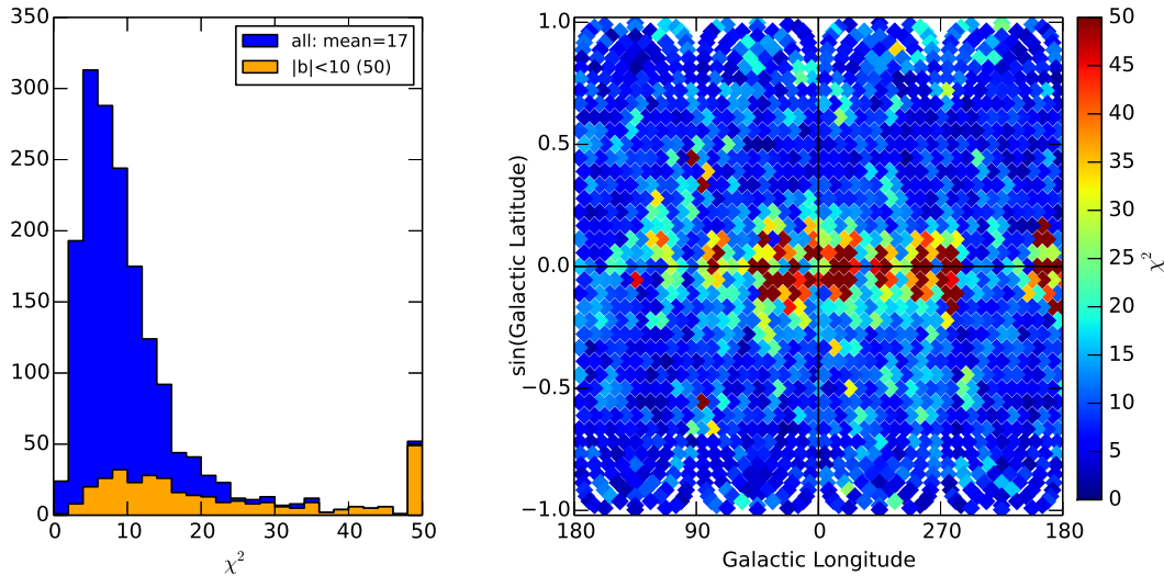
Fig. 2.— Distributions of the \chi^2 measure of consistency of the measured spectrum of each RoI with the model (capped at 50). Left: histogram highlighting the low-latitude subset. Right: distribution of the values over the sky.
