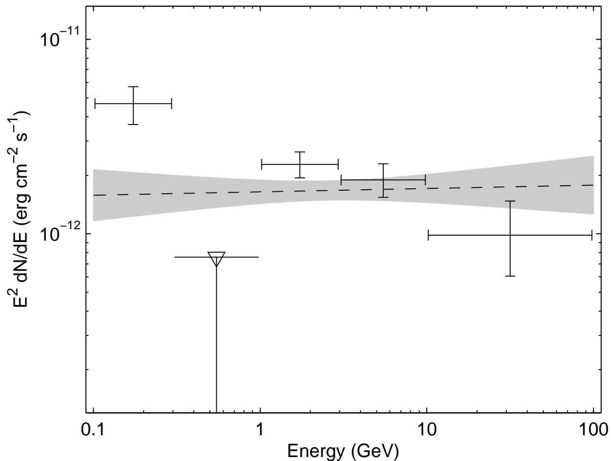
Fig. 9.— Spectral energy distribution of 3FGL J1226.9–1329 (PMN J1226–1328) flagged with bad spectral fit quality (Flag 10 in Table 3). The first two points deviate from the power-law fit. This source is within 1.3^\circ of the much brighter pulsar PSR J1231–1411 so it is confused with it (within r_{68} ) below 600 MeV.
