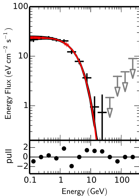
Fig. 3.— The spectral energy distribution for a typical source, in this case PSR J1459–6053, as measured by the pointlike analysis. The lower plot shows the pulls , defined as the square root of the difference 2\Delta \log \mathcal{L} between the fitted flux and the spectral model in each energy band, signed with the residual. The points with error bars reflect the dependence of the likelihood on the flux for each energy band, combining Front and Back , while the curve is the result of the fit to all the energy bands.
