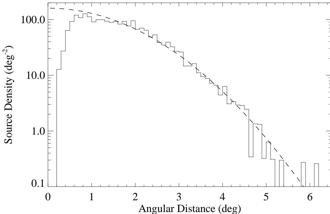
Fig. 13.— Distribution of nearest-neighbor distances for 3FGL sources at |b| > 10^\circ . The dashed curve was derived as described in Abdo et al. (2010d, 1FGL). It is the distribution expected if sources could be detected at arbitrarily small angular separations. The dashed curve is normalized to match the total observed number of sources for separations > 0.8 (2035). This corresponds to an expected true number of sources (extrapolated down to 0 separation) of 2336 at |b| > 10^\circ .
