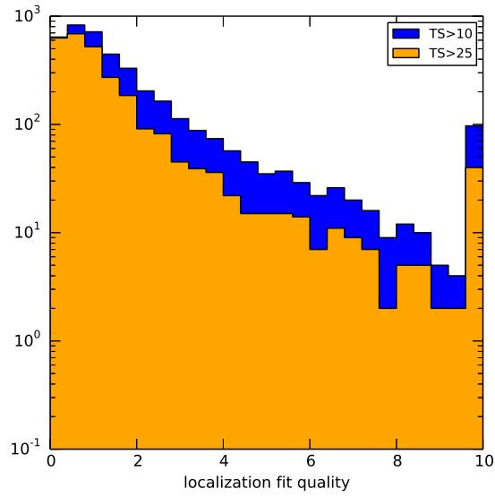
Fig. 6.— The distribution, in the preliminary source list, of the localization quality LQ (capped at 10).
