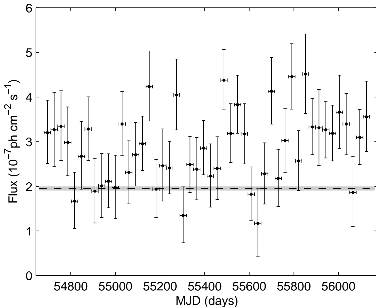
Fig. 11.— Light curve of 3FGL J1616.2–5054e (HESS J1616–508). That is an extended source that should not be variable. Indeed the monthly fluxes are compatible with a constant, but not with the flux extracted over the full four years (dashed line with gray-shaded uncertainty). That inconsistency is due to a remaining difference between binned and unbinned likelihood fits affecting only extended sources.
