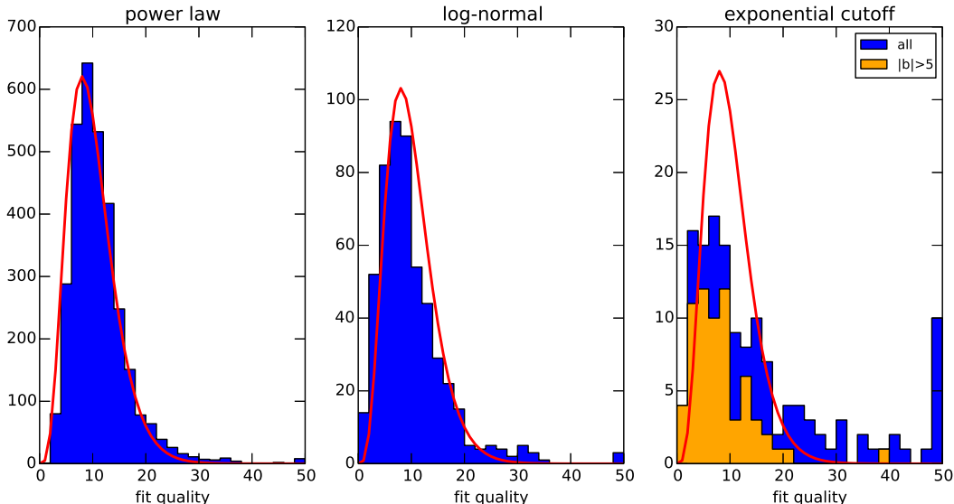
Fig. 4.— Distributions of the spectral fit quality (capped at 50). Left: sources fit with a power-law spectrum; Center: sources fit with a log-normal; Right: sources fit with a power law with exponential cutoff. All are overlaid with the \chi^2 distribution with 10 degrees of freedom.
