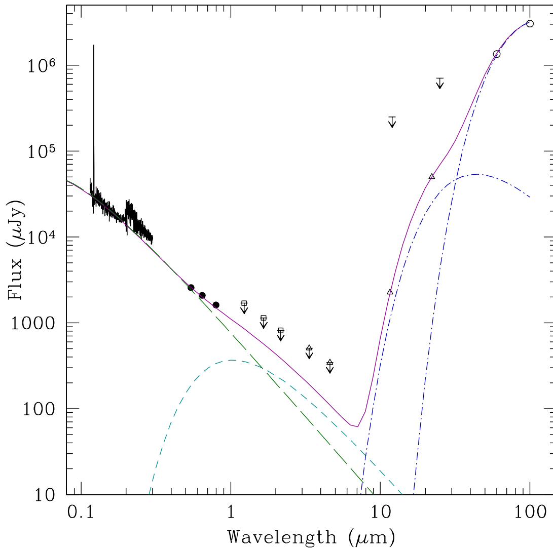
Fig. 1.— The spectral energy distribution plot for the CS of Abell 65. The IUE spectra, V , R , and I magnitudes ( solid circles ) at minimum light, 2MASS J , H , and K magnitudes ( open squares ), WISE fluxes ( open triangles ), and IRAS fluxes ( open circles ). All fluxes have been de-reddened assuming E(B - V) = 0.20 . Also shown are model blackbody curves for our resulting CS, companion, and dust component, as well as the combined curve. These are shown without any irradiation contribution, thus should approximately represent the system at minimum light.
