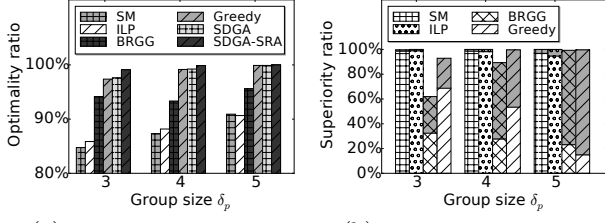
(a) Optimality ratio (T) (b) Superiority ratio (T)
