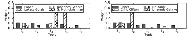
(a) ILP (Score = 0.77) (b) BRGG (Score = 0.64)
