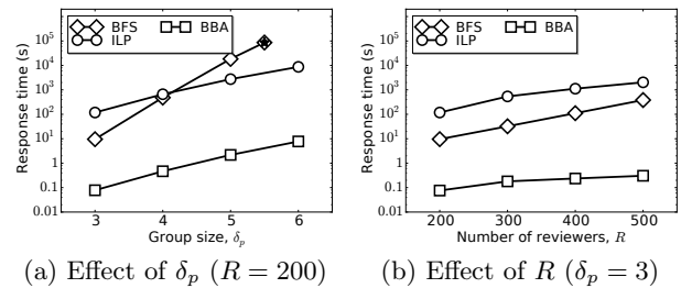
Figure 9: Scalability evaluation of JRA
