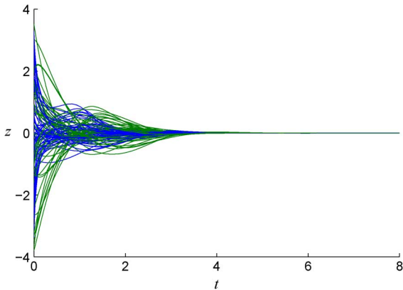
Fig. 2. Example 1. Trajectories of robust synchronization.
