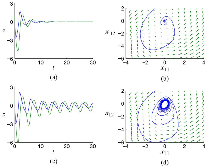
Fig. 1. Example 1. Hopf bifurcation of coupled M-G jet engines.
