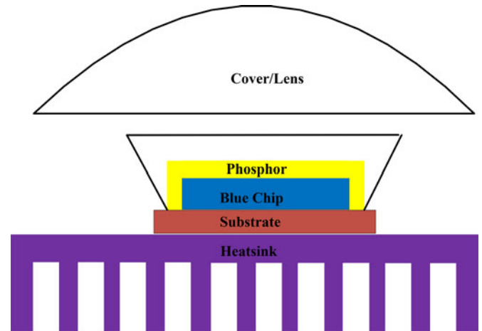
Fig. 2. Detailed inside view of the function stages of an LED package.
