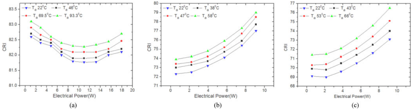
Fig. 10. Measured color rendering index (CRI) with the LED bulb in the downward position. (a) Shineon LED. (b) Cree-XRE LED. (c) Osram-W5AP.
