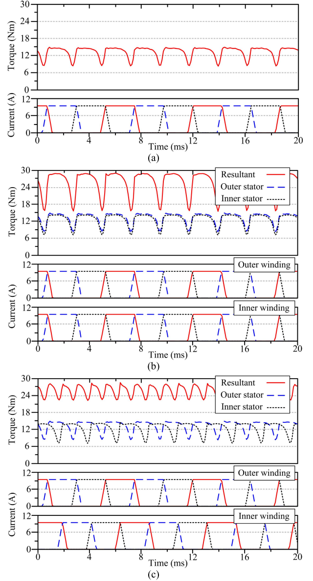
Fig. 4. Rated torque waveforms. (a) MSR. (b) DS-MSR. (c) MO-DS-MSR.
