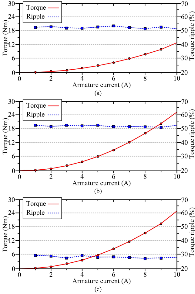
Fig. 3. Average torque and torque ripple performances. (a) MSR. (b) DS-MSR. (c) MO-DS-MSR.
