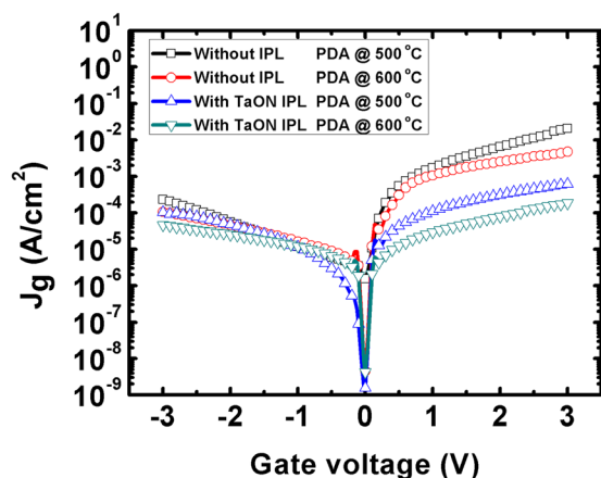
FIG. 3. J_g - V_g characteristics of GaAs MOS capacitors with/without TaON, annealed at 500 and 600 °C.
