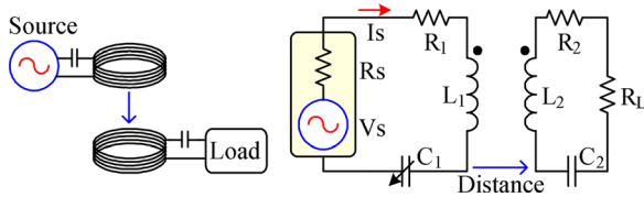
FIG. 2. Basic circuit topology for WPT on Mars.
