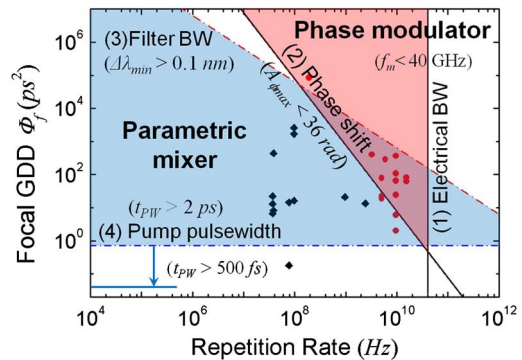
Fig. 5. Effect of repetition rate on the focal GDD range for two time-lens mechanisms. Solid line: constraints on the phase modulator (1) and (2). Dashed-dotted line: constraints on the parametric mixer (3) and (4). Two sets of dots correspond to the relations shown in Fig. 1.
