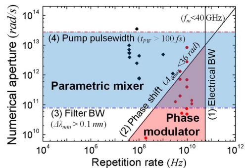
Fig. 7. Effect of repetition rate on the temporal NA performance for two time-lens mechanisms. Solid line: constraints on the phase modulator (1) and (2). Dashed-dotted line: constraints on the parametric mixer (3) and (4). Two sets of dots correspond to the relations shown in Fig. 1.
