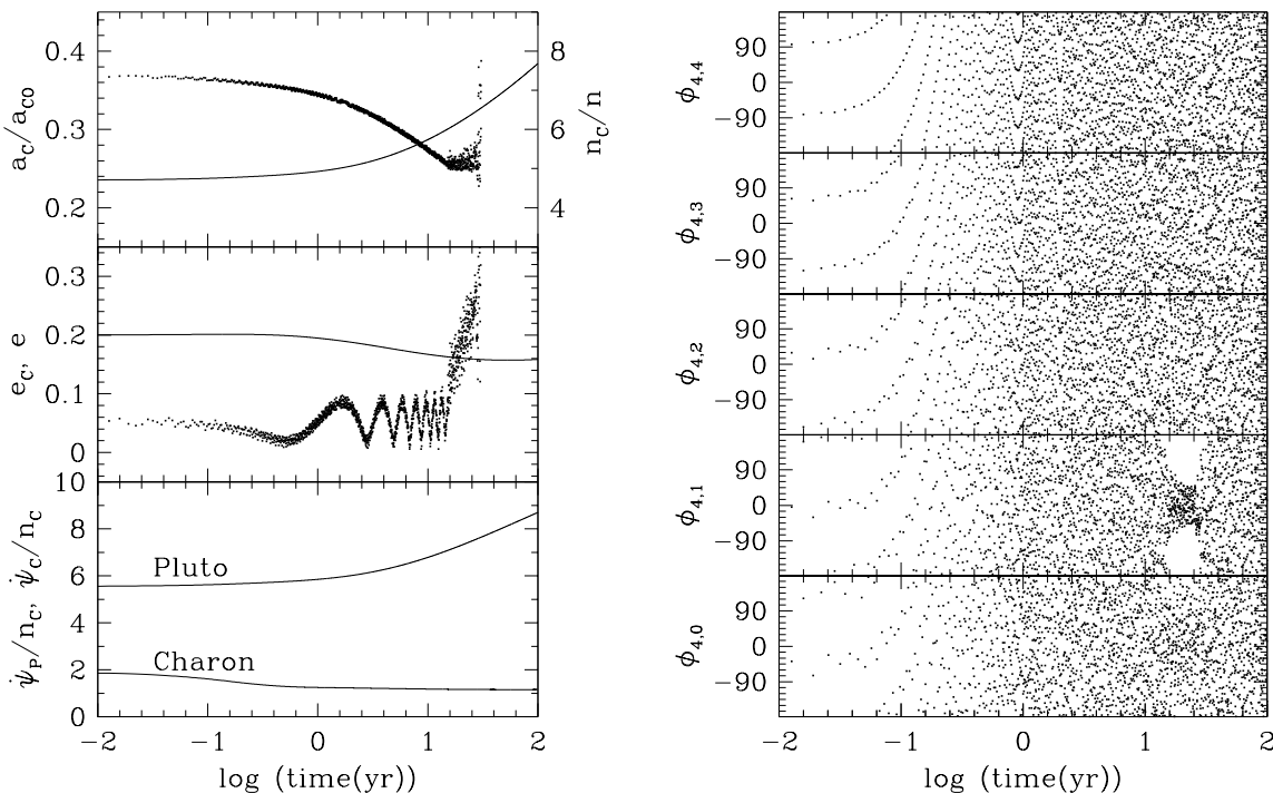
Fig. 2.— Example of a test particle captured into a single 5:1 Lindblad resonance with Charon in the constant \Delta t model. The panels show the evolution of Charon’s orbital semimajor axis a_C (in units of its current semimajor axis a_{C0} ) and eccentricity e_C and the spin angular velocities \dot{\psi}_i of Pluto and Charon (in units of Charon’s mean motion n_C ) as lines, and the evolution of e , the ratio of mean motion n_C/n , and the resonance variables \phi_{4,l} of the test particle as dots. e increases when \phi_{4,1} is librating, and the test particle becomes unstable.
