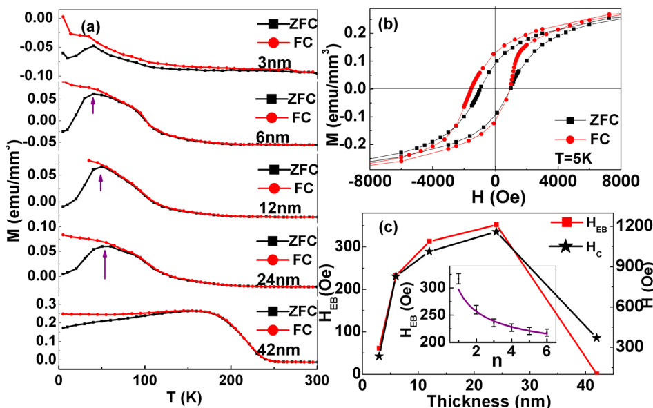
FIG. 3. (a) Temperature dependence of magnetizations with ZFC and FC processes for L3, L6, L12, L24, and L42, respectively. (b) Hysteresis loops of L24 at 5K measured after zero-field cooling and field cooling in 500 Oe field. (c) Thickness dependence of H_{EB} and H_c at 5K. The inset is the number of filed cycles n dependence of H_{EB} for L12. The cooling field is set to 500 Oe. Solid line shows the best fit to the data for n > 1 .
