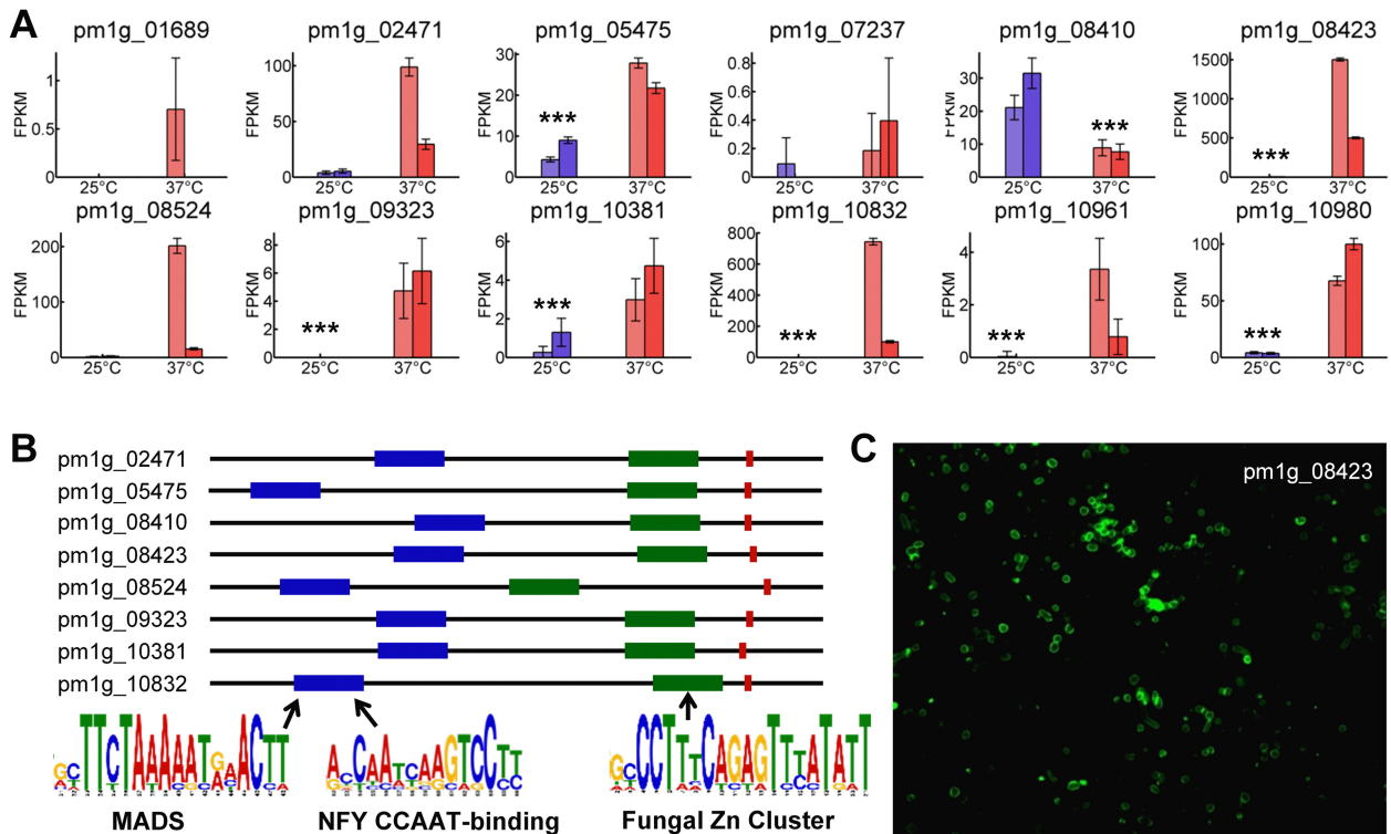
FIG 4 Expression levels of P. marneffii MP1 domain genes and their regulatory regions. (A) Expression levels of 12 MP1 domain genes at 25 versus 37°C (see Materials and Methods for details). (B) Putative transcription factor binding sites in 5' regulatory regions. The positions of binding motifs are indicated with the blue and green bars and labeled with the subtype name of transcription factors: (i) MADS, (ii) NFY CCAAT binding, and (iii) fungal Zn cluster. The position of the TATA box is indicated by the red bar. (C) Indirect immunofluorescent staining with antibodies to Mp1p (pm1g_08423) at 37°C.
