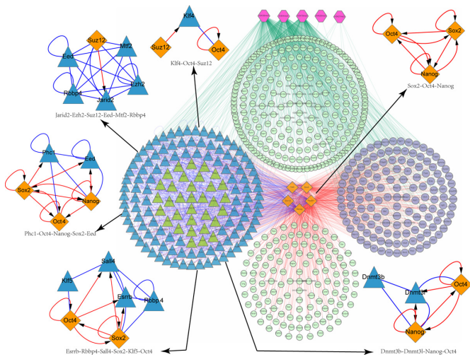
Figure 2. A post-translational hierarchical gene down-regulatory network in mouse ES cell. Triangle nodes represent proteins, with blue ones referring to those also targeted by TFs or epigenetic modifications and green ones referring to those only interacting with proteins. Blue non-directional edges are protein–protein interactions. Red and green arrow edges represent target genes of TFs and epigenetic modifications, respectively. Diamond and hexagon nodes represent TFs and epigenetic modifications, respectively. The six subgraphs represent the selected interactions among TFs, cofactors, epigenetic enzymes and other proteins in ES cell.
